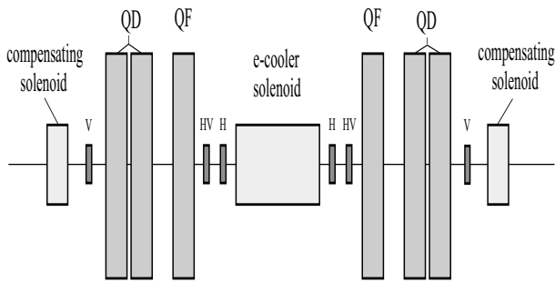
Figure 2: Schematic view of the AD electron cooling insertion.
