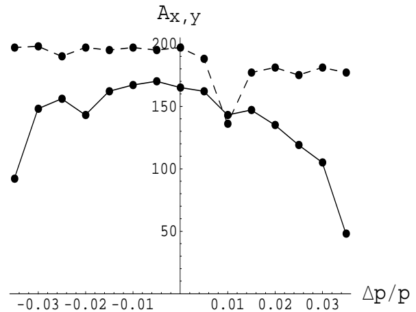
Figure 4: The horizontal and the vertical AD acceptances (solid and dashed line respectively) versus momentum deviation at injection energy. The measurements were done at early stage of the commissioning.
