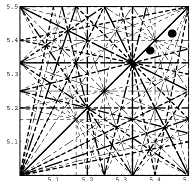
Figure 1: AD tune diagram ( Q_x, Q_y ) with two working points now in operation. Resonances up to 6 order are shown.
