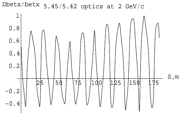
Figure 5: Relative deviations of the horizontal beta function from the designed one due to the gradient errors.
