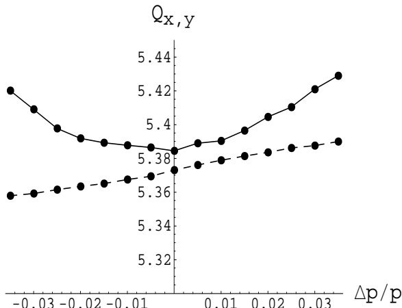
Figure 3: The horizontal and the vertical AD tune at injection energy (solid and dashed line respectively) versus momentum deviation.
