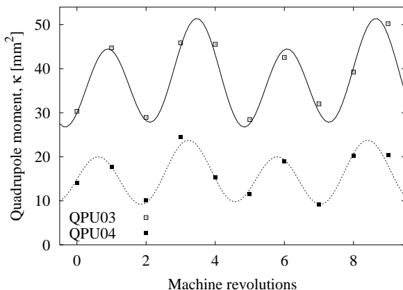
Figure 3: Theoretical expression for the quadrupole moment fitted to measured data. Ten turns (20 data points) were used to determine the ten free parameters (emittances, betatron and dispersion mismatches, and the tunes).
