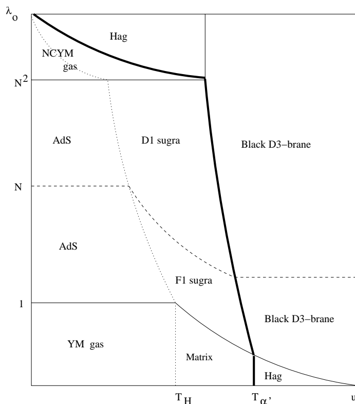
Figure 3: The phase diagram of the full (D3,F1) bound state in \lambda_o versus the radial energy variable u , including the maximum temperature line that appears when the NCOS decoupling is not complete. To the right of the thick line one finds true Hagedorn phases or black-brane phases with negative specific heat. In the exact NCOS limit T_{\alpha'} \rightarrow \infty and this thick line is pushed to infinite energies. The region of large energies u > T_H and low NCOS coupling (below the dashed S -duality line) has universal features, independent of the Dp -brane dimension.
