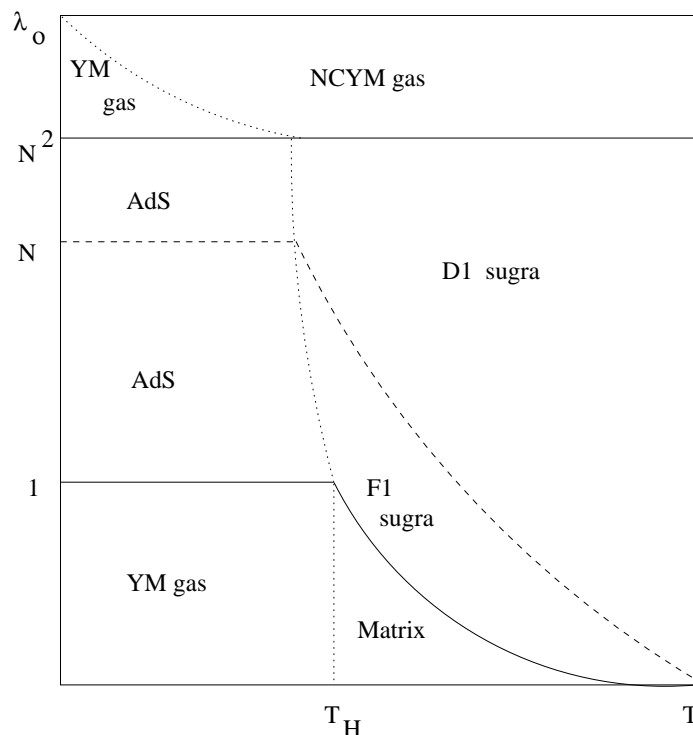
Figure 2: The four-dimensional phase diagram in NCOS variables. The conventions for the transition lines are the same as in figure 1. The notations ‘F1 sugra’ and ‘D1 sugra’ refer to the fact that the corresponding metrics are well approximated by those of smeared one-branes.
