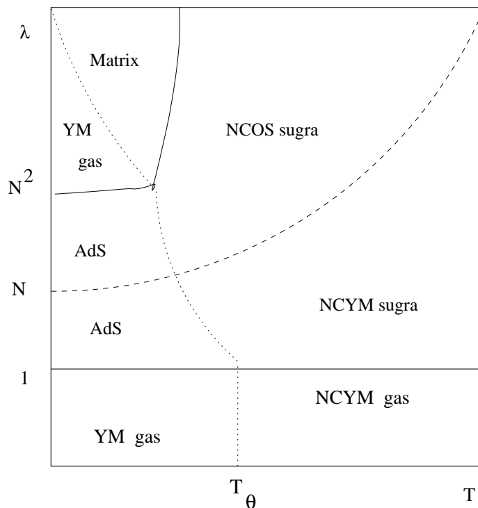
Figure 1: The four-dimensional phase diagram in NCYM variables. Full lines denote crossovers based on the correspondence principle. The dashed line is the S-duality transition. The dotted lines denote the onset of noncommutative effects and T_\theta \equiv 1/\sqrt{\theta} .
