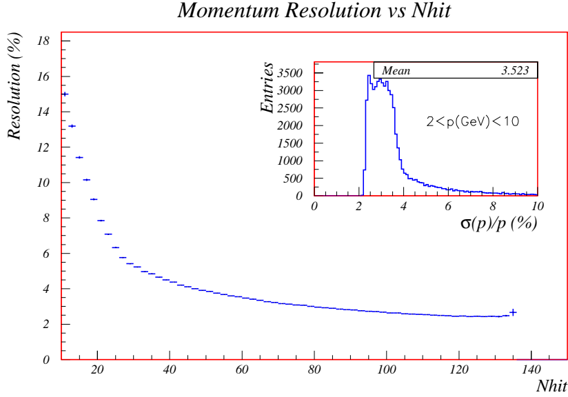
Fig. 22. Momentum resolution as a function of the track length (number of hits in the fiducial volume of drift chambers). The insert shows the distribution of the number of tracks at a given resolution.
