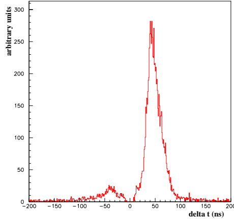
Fig. 16. Example of the time difference (in ns) between a second hit on the same wire and the hit included in a given track.
