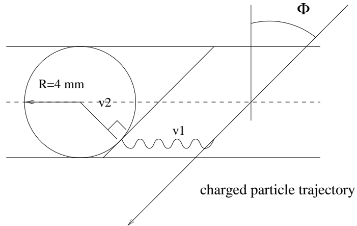
Fig. 10. A model used to describe the drift of electrons in the drift cell.
