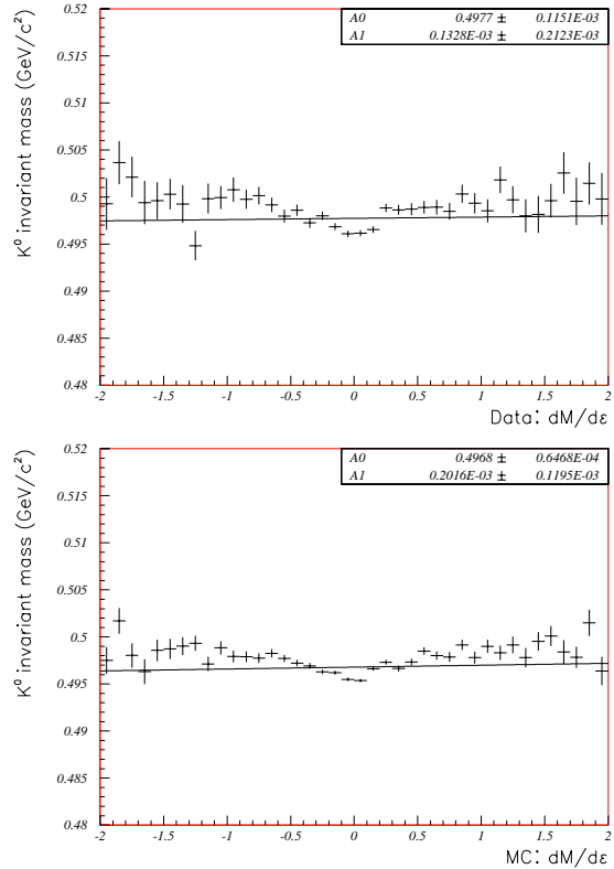
Fig. 26. Invariant mass as a function of \partial M/\partial \varepsilon for both data and Monte Carlo. The result of the fit is also shown.
