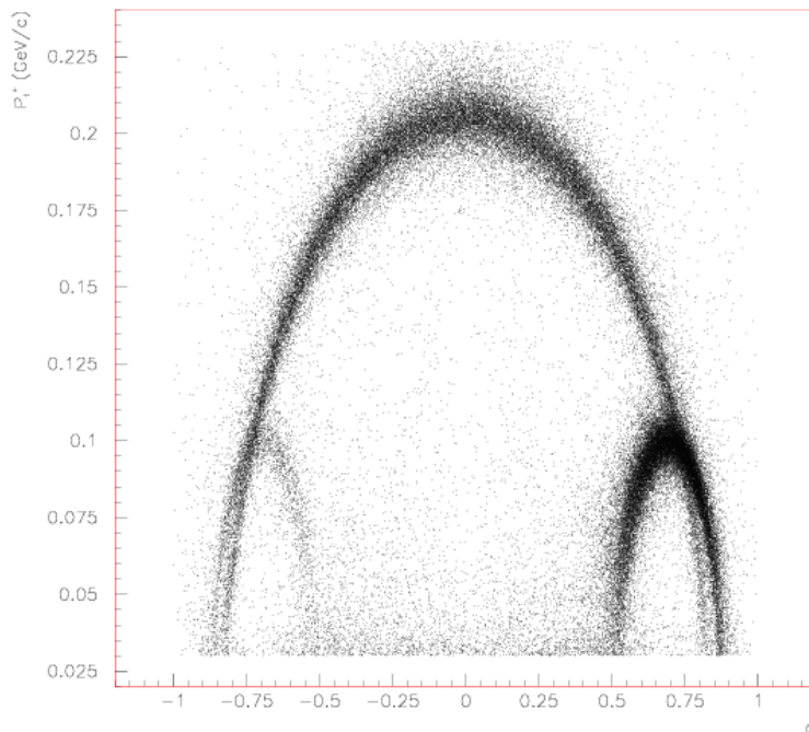
Fig. 24. Armenteros' plot for reconstructed V^0 's: K_s^0 's cluster on the large central ellipse, \Lambda 's on the small right ellipse and the smaller sample of \bar{\Lambda} 's on the left one.
