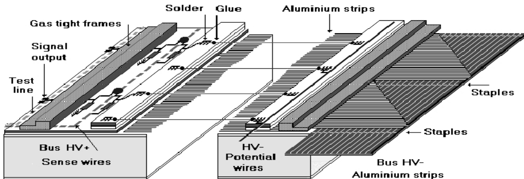
Fig. 3. A cut view of a panel equipped as a Y plane.
