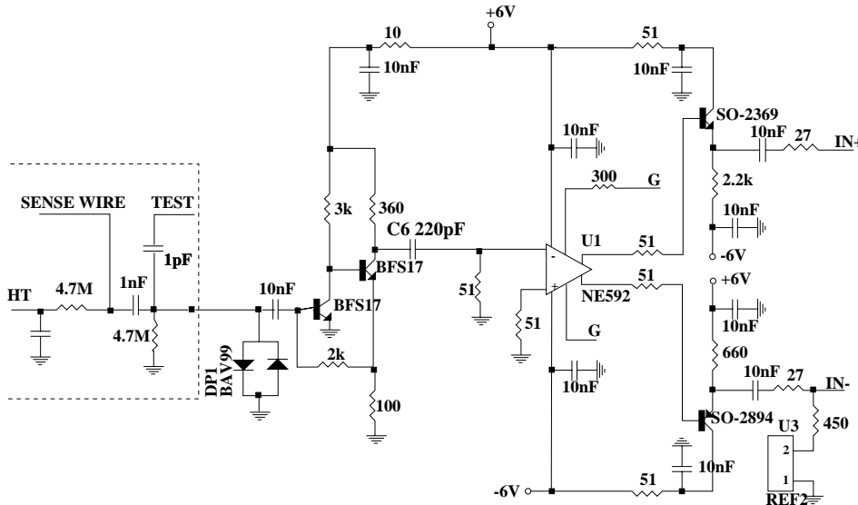
Fig. 6. Schematic diagram of the preamplifier.
