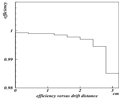
Fig. 14. The dependence of the hit finding efficiency on the track position in the drift cell.
