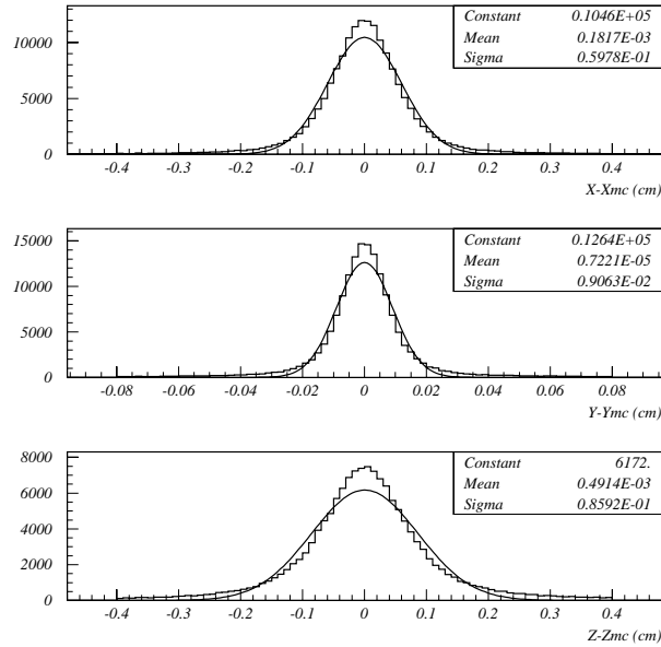
Fig. 21. The vertex position resolution for reconstructed \nu_\mu CC MC events. The resolution is 600 \mu\text{m} , 90 \mu\text{m} and 860 \mu\text{m} for x , y and z respectively.
