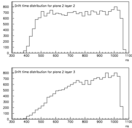
Fig. 9. Drift time distribution as measured by the cosmic test setup. Top: for correctly aligned strip bands. Bottom: for misaligned ones.
