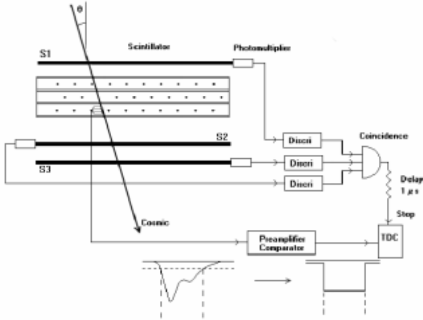
Fig. 8. The cosmic test setup.
