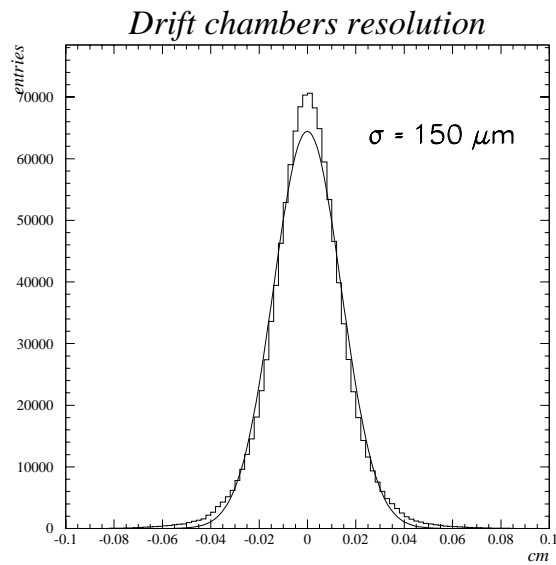
Fig. 11. Residuals for a sample of straight tracks in the drift chambers.
