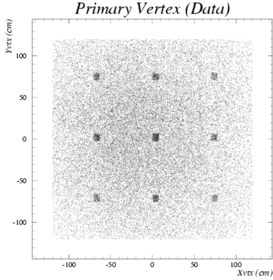
Fig. 19. The positions of reconstructed neutrino interaction vertices from experimental data in a plane perpendicular to the beam direction; see text for details.
