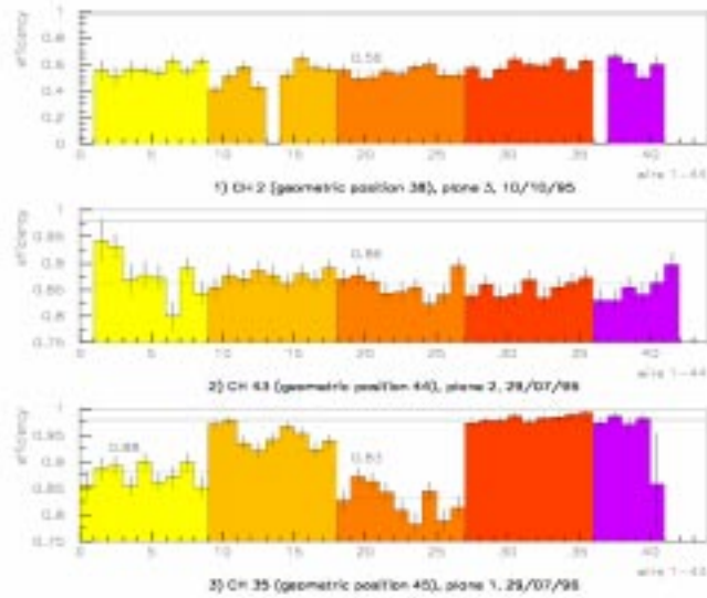
Fig. 15. Examples of hardware efficiency losses for some pathological drift chamber planes. The horizontal solid line shows an efficiency \varepsilon = 0.98 for normal chambers. The different shaded areas indicate different layers of cathode strips. (1) for planes with short circuits between strips: the efficiency loss is \approx 42\% ; (2) for disconnected field wires: the efficiency loss is \approx 12\% ; (3) for misaligned strip layers: the efficiency loss is \approx 10 \div 15\% .
