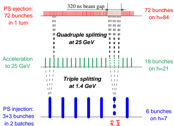
Fig. 1: Multiple splitting scheme for the LHC beam. “Quadruple” splitting means two steps of double splitting.
