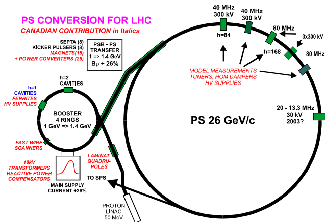
Fig. 2: Major hardware upgrades in the PS complex.
