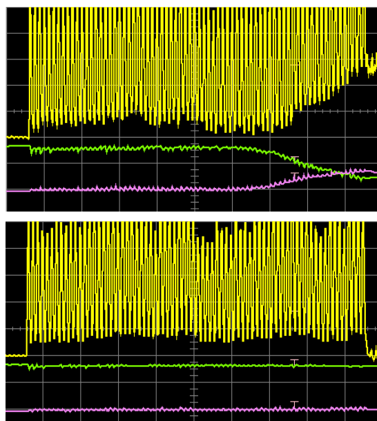
Fig. 8: Baseline drift of the signal from an electrostatic pick-up in the PS-SPS transfer line (TT2) due to electron cloud build-up: (top) solenoid off, (bottom) solenoid ( \sim 50 G) on. On each oscillogram, from top to bottom: Sum-signal, \Delta x , \Delta y . The beam features 72 bunches, spacing 25 ns, length 4 ns.
