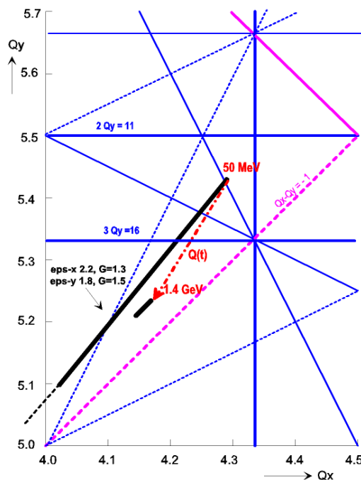
Fig. 3: PS Booster tune diagram with stopbands, time-varying tunes Q(t) , and space-charge tune-spread at injection and ejection energies. N=1.4 \times 10^{12} protons/ring, bunching factor 0.55, \epsilon_{x,y} normalised rms emittances.
