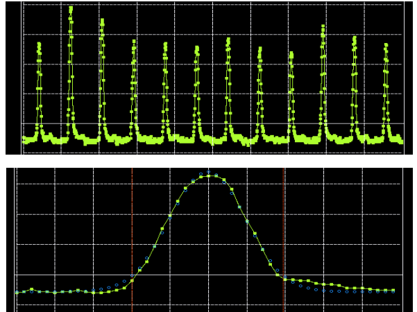
Fig. 6: Twelve out of 72 bunches on the last turn of the PS (top, 30 ns/div); zoom on one bunch (1 ns/div).
