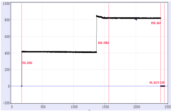
Fig. 4: Intensity of the PS ring (in units of 10^{10} protons) vs. time (in ms).
