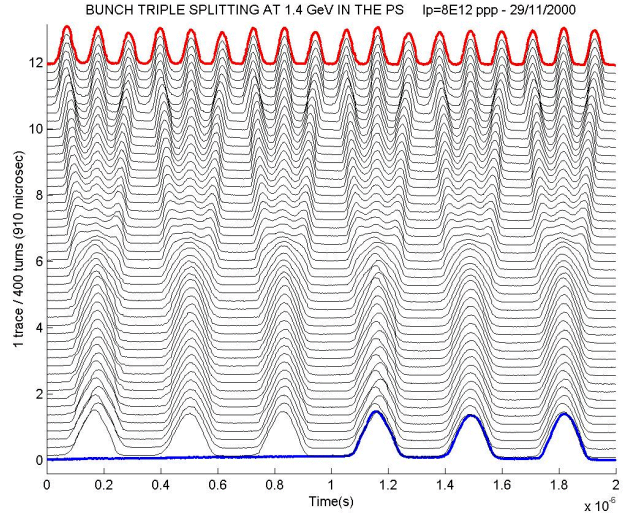
Fig. 5: Bunch triple-splitting of 6 PSB bunches into 18 in the PS at 1.4 GeV. The process takes about 40 ms.
