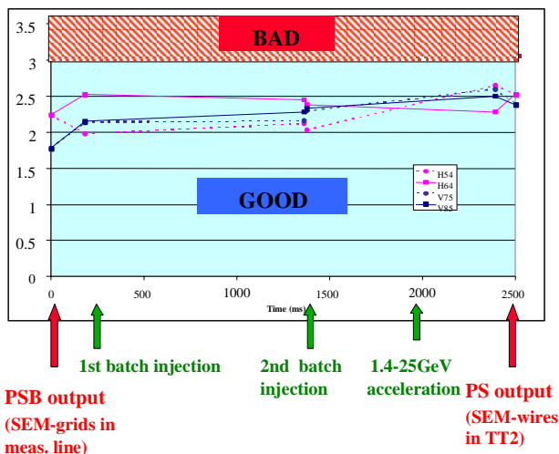
Fig. 7: Evolution of the normalised rms emittances from PSB exit to PS extraction (H=horizontal, V=vertical). Measurements in TT2 were done without bunch compression.
