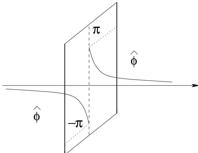
Figure 1: Schematic representation of the solution profile of the \hat{\phi} field as a function of the coordinate perpendicular to the domain wall.
