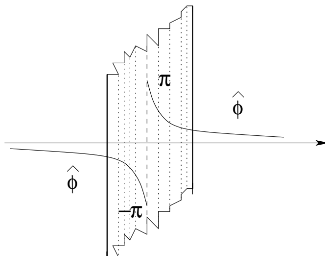
Figure 2: Schematic representation of the solution profile of the \hat{\phi} field with a “rough” domain wall profile.
