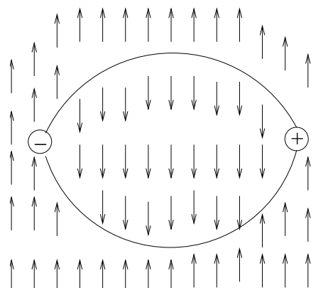
Figure 5: The Ising domain created by the two strings connecting the positions of W^+ and W^- particles. For static particles the configuration propagates in the time direction, perpendicular to the plane of the page.
