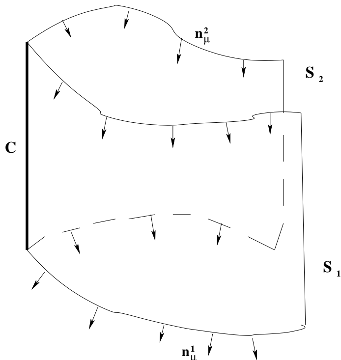
Figure 4: The two surfaces S_1 and S_2 along which the current j_\mu is non-vanishing. The surfaces come together at the line C which is the world-line of the W boson.
