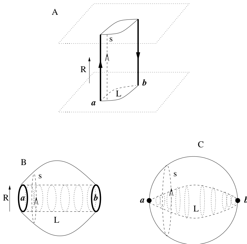
Figure 7: The D0 brane-anti-brane ( W^+ - W^- ) pair with two strings connecting them conformally transformed into a string world-sheet with two “double vortices”.
