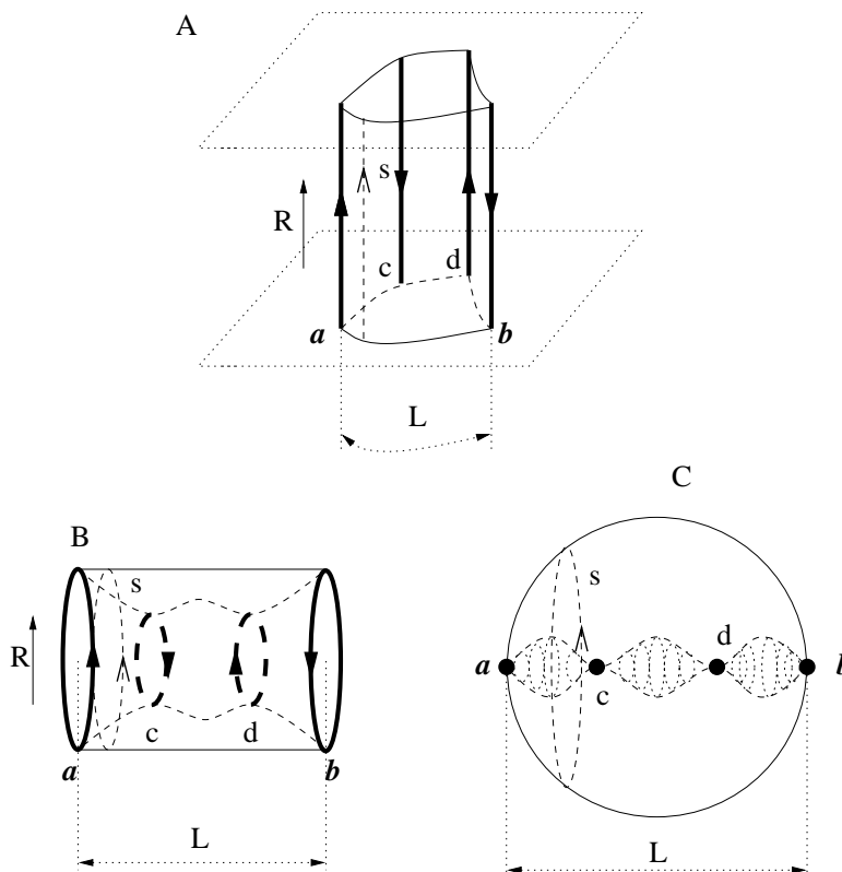
Figure 8: Four branes connected by strings. Such configurations become important above the transition.
