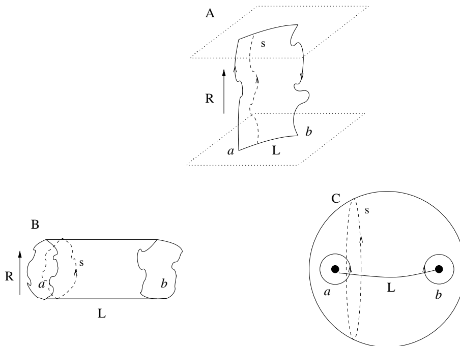
Figure 6: The open string world-sheet conformally transformed into a closed string world-sheet with a vortex-anti-vortex pair. L is the length of the string, a and b are locations of the vortex and the anti-vortex on the world-sheet and R represents the compact dimension.
