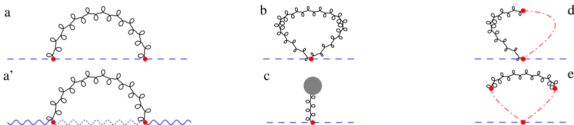
Figure 1: One-loop gravitational corrections to the pole mass of a scalar on a brane from gravitons (diagrams a,b,c ) and from graviton/branon mixing (diagrams d,e ) at zeroth order in the brane tension. The mass of a vector particle on a brane also gets corrections from vector-Goldstone-graviton vertices (diagram a' ). Gravitons (branons, scalars, vectors, Goldstones) are drawn as pig-tail (dot-dashed, dashed, wavy, dashed-wavy) lines.
