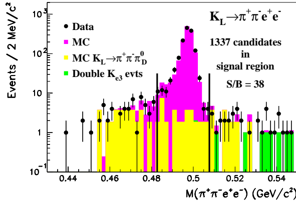
Figure 1. Invariant mass distribution of K_L \rightarrow \pi^+\pi^-e^+e^- candidate events.
