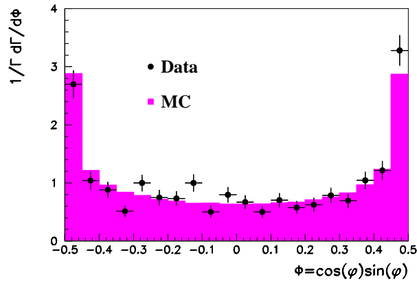
Figure 5. Acceptance corrected \sin(\varphi)\cos(\varphi) distribution of K_S \rightarrow \pi^+\pi^-\pi^0 candidate events (1998+1999 data).
