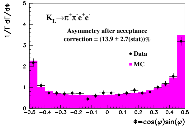
Figure 2. Acceptance corrected \sin(\varphi)\cos(\varphi) distribution of K_L \rightarrow \pi^+\pi^-e^+e^- candidate events.
