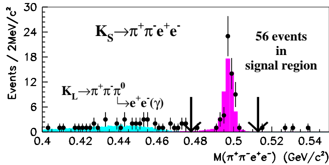
Figure 3. Invariant mass distribution of K_S \rightarrow \pi^+\pi^-e^+e^- candidate events (1998 data).
