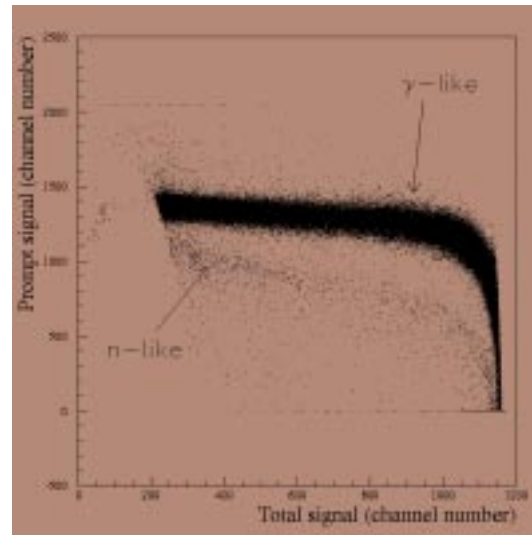
Fig. 4. Second pulse shape discrimination (PSD2) for the N1 detector. Prompt signal amplitude vs. total signal amplitude.
