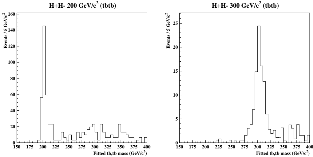
FIGURE 1. Fitted charged Higgs boson mass for H^+H^- \rightarrow t\bar{t}b\bar{b} with M_{H^\pm} = 200 \text{ GeV}/c^2 (left plot) and M_{H^\pm} = 300 \text{ GeV}/c^2 (right plot). The histograms are normalized to 500 \text{ fb}^{-1} integrated luminosity and 100% branching ratio into the analyzed decay mode.
