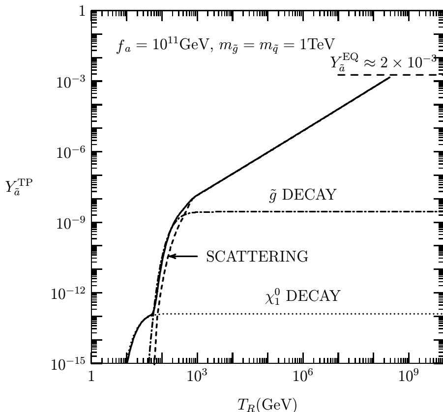
Figure 2: Y_a^{\text{TP}} as a function of T_R for representative values of f_a = 10^{11} GeV and m_{\tilde{q}} = m_{\tilde{g}} = 1 TeV.
