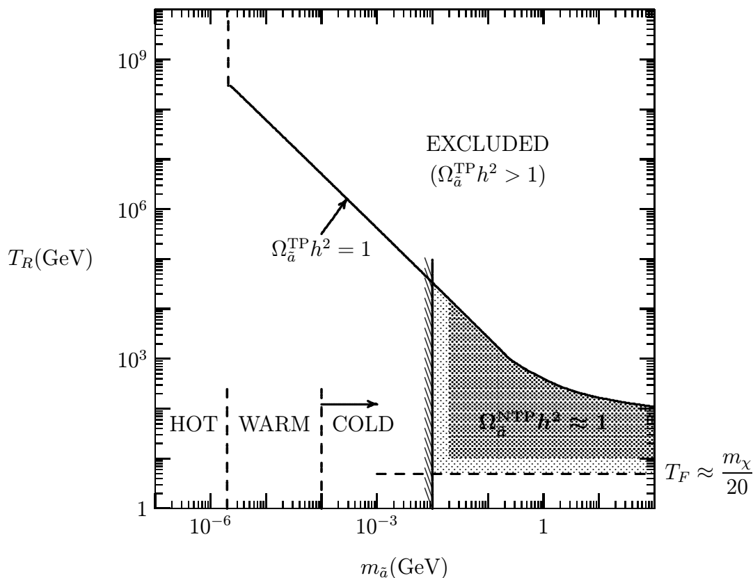
Figure 5: The solid line gives the upper bound from thermal production on the reheating temperature as a function of the axino mass. The dark region is the region where non-thermal production can give cosmologically interesting results ( \Omega_{\tilde{a}}^{\text{NTP}} h^2 \simeq 1 ) as explained in the text. We assume a bino-like neutralino with m_\chi = 100 GeV and f_a = 10^{11} GeV. The region of T_R \gtrsim T_f is somewhat uncertain and is shown with light-grey color. A sizeable abundance of neutralinos (and therefore axinos) is expected also for T_R \lesssim T_f [50] but has not been calculated. The vertical light-grey band indicates that a low range of m_{\tilde{a}} corresponds to allowing SM superpartner masses in the multi-TeV range, as discussed in the text. The division of hot, warm and cold dark matter as a function of the axino mass shown in the lower left part is for axinos from non-thermal production.
