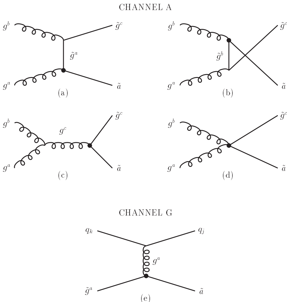
Figure 1: Feynman diagrams contributing to channels A and G in table 1. Thick dot denotes effective axino couplings to ordinary colored particles.
