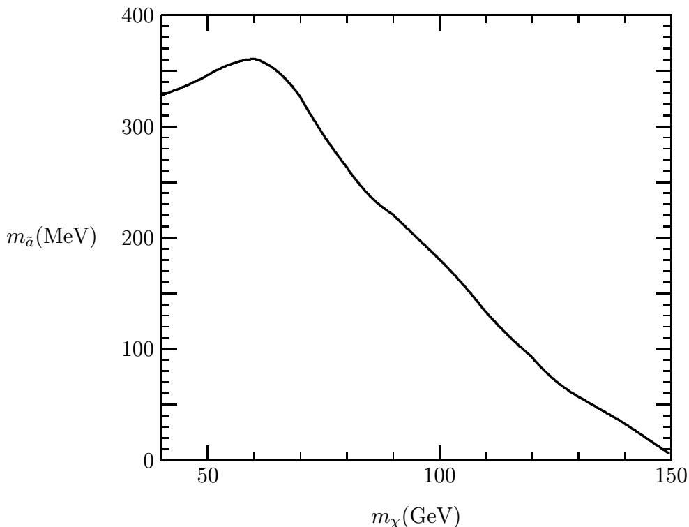
Figure 4: Lower bound on the axino mass from considering hadronic showers according to the condition (5.24), for C_{aYY}Z_{11} = 1 and f_a/N = 10^{11} GeV. The bound disappears for m_\chi = 150 GeV when the lifetime drops below 0.1 sec.
