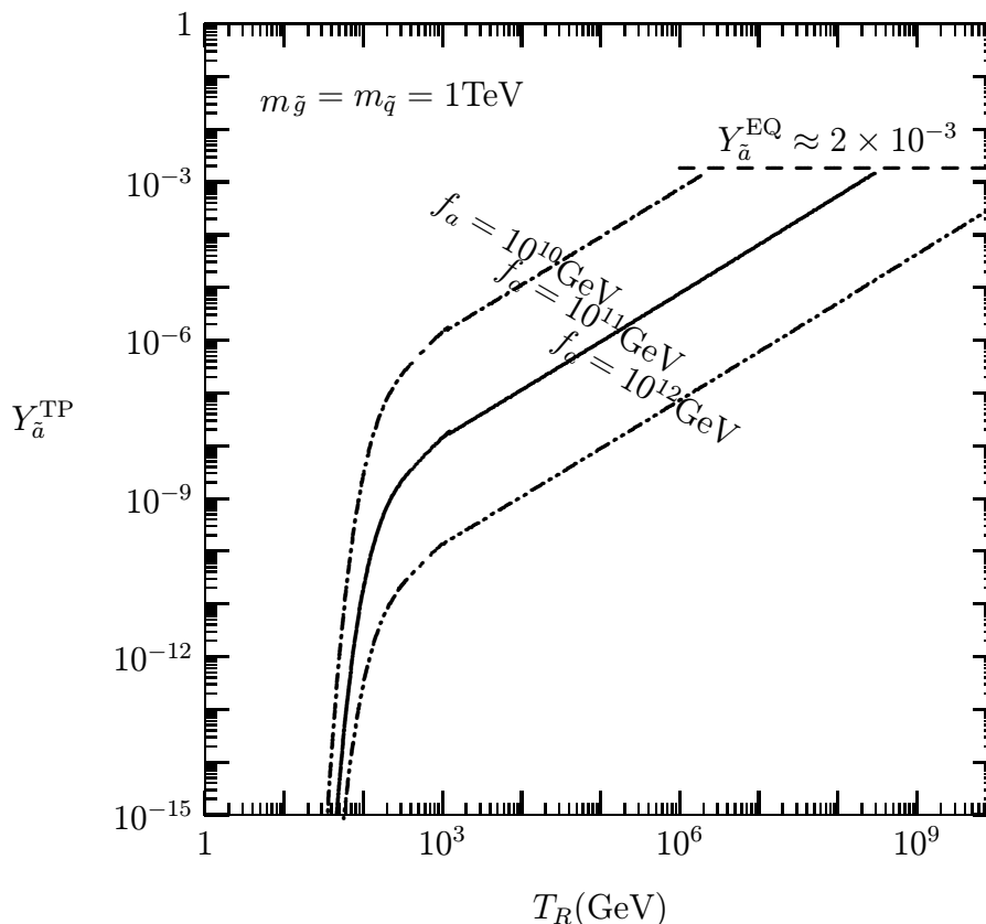
Figure 3: Y_{\tilde{a}}^{\text{TP}} as a function of T_R for representative values of f_a and m_{\tilde{q}} = m_{\tilde{g}} = 1 \text{ TeV} .
