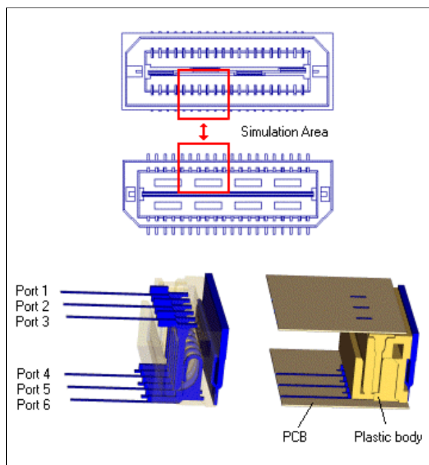
Figure 6: 3D connector model.
