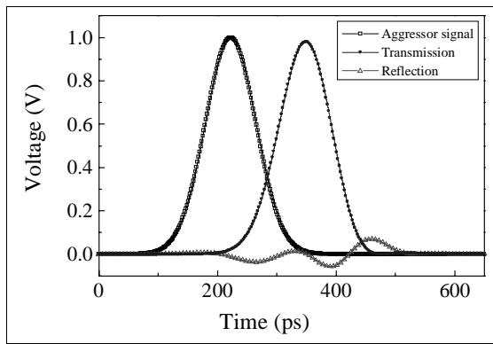
Figure 7: Time-domain connector transmission results.
