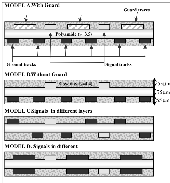
Figure 4: Different signal-ground track configurations.
