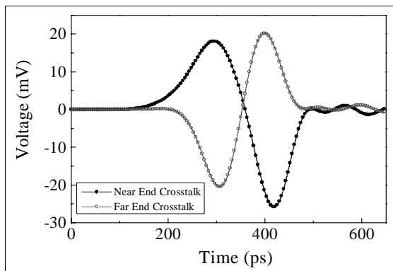
Figure 8: Near-end (port 1) and far-end (port 4) crosstalk
