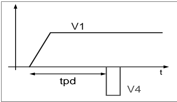
Figure 2: Forward crosstalk (V4) in the far-end of the victim line for an aggressor signal (V1).
