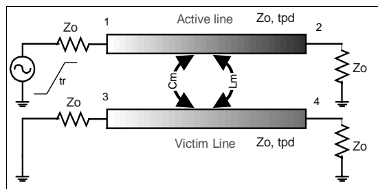
Figure 1: Crosstalk scenario. C_m models the capacitive crosstalk; L_m models the inductive one.
