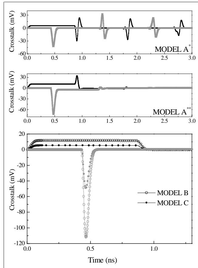
Figure 5: Far-end and near-end crosstalk for the different configurations.
