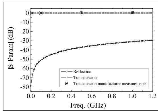
Figure 9: Frequency-domain connector transmission results.
