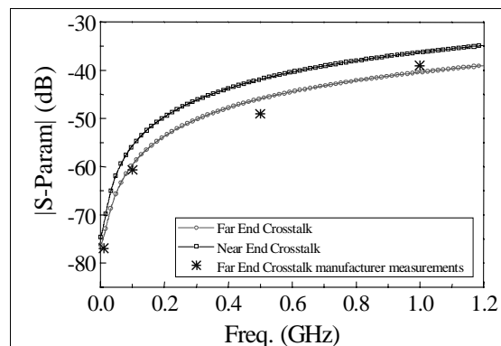
Figure 10: Near-end ( |S_{21}| ) and far-end ( |S_{24}| ) crosstalk
