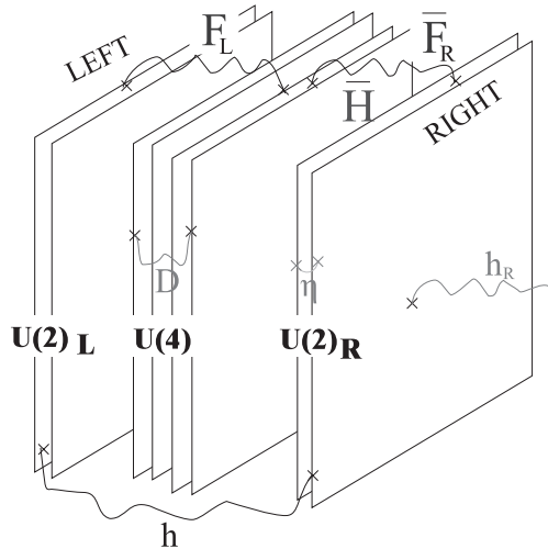
Figure 1: Assignment of the Standard model particles in a D-brane scenario with gauge group U(4)_C \times U(2)_L \times U(2)_R . The standard model particles are assigned to F_L = Q + L , \bar{F}_R = u^c + d^c + e^c + \nu^c and the electroweak Higgs to h = H_u + H_d . They are all represented by strings having both their ends attached to two different branes. The PS breaking Higgs scalars ( \bar{H} ) are similar to \bar{F}_R . In gray we represent particles whose presence is not required in all versions of the model. These are the extra scalar triplets D = \tilde{d} + \tilde{d}^c , the right-handed doublets h_R and the singlet \eta .
