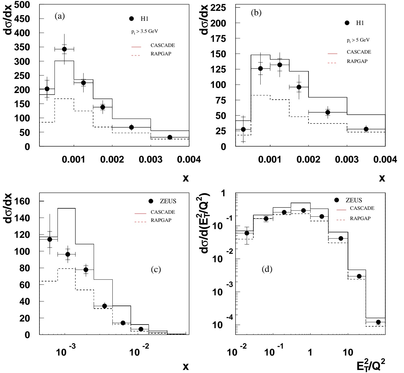
Figure 5: The cross section for forward-jet production obtained from the Monte Carlo CASCADE at hadron level (solid line); (a – c) The cross section for forward-jet production as a function of x , for different cuts in p_t compared to H1 data [43] (a – b) and compared to ZEUS data [44] (c); (d) The cross section for forward-jet production as a function of E_T^2/Q^2 compared to [45].
