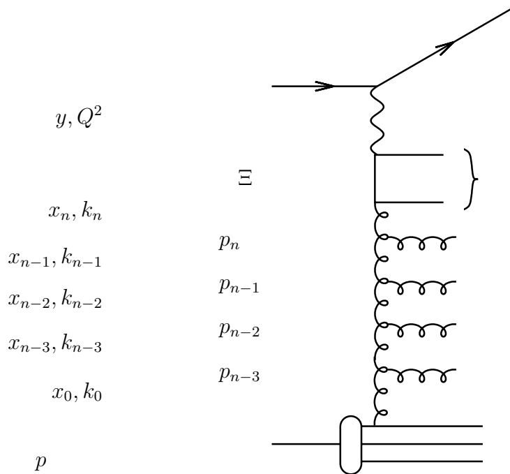
Figure 1: Kinematic variables for multi-gluon emission. The t -channel gluon four-vectors are given by k_i and the gluons emitted in the initial state cascade have four-vectors p_i . The upper angle for any emission is obtained from the quark box, as indicated with \Xi .
