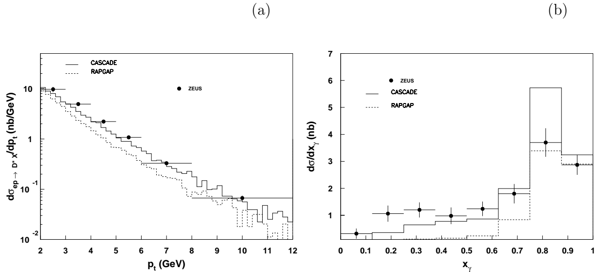
Figure 7: The differential cross sections of D^* photo-production [49] for d\sigma/dp_t^{D^*} (a) and d\sigma/dx_\gamma (b). The solid line shows the prediction from CASCADE while the dashed line shows the prediction from RAPGAP.
