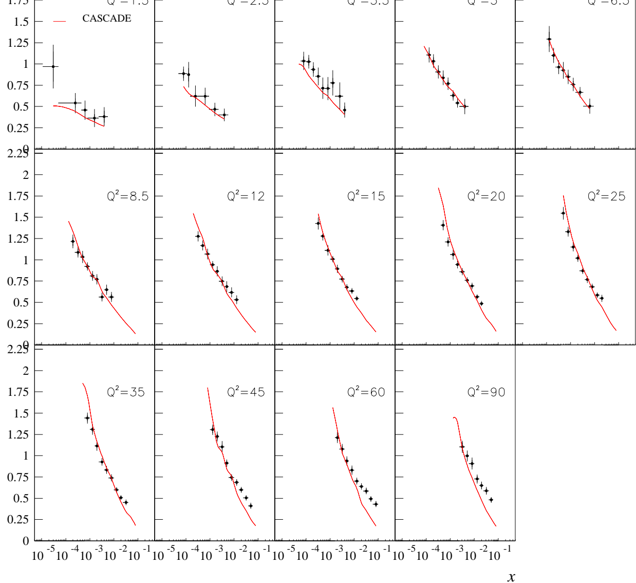
Figure 4: Comparison of the structure function F_2 as obtained from the backward evolution Monte Carlo CASCADE with H1 data [42].
