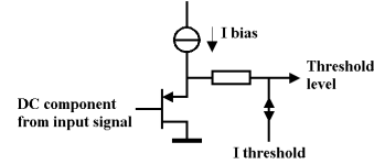
Figure 4: Adder
