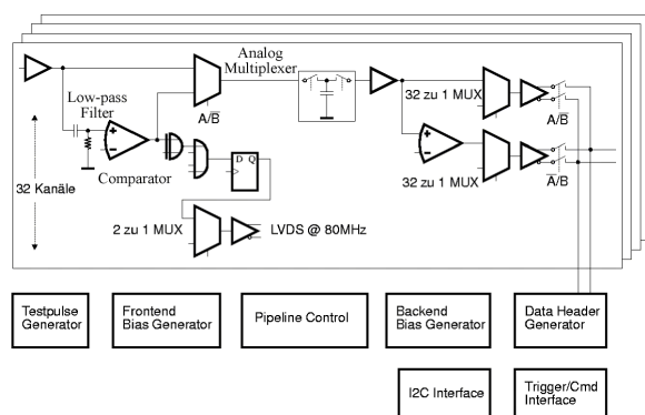
Figure 1: Block diagram of the Beetle chip
