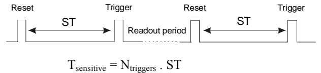
Figure 6: Definition of ST for the pipeline logic FIFO and control logic
