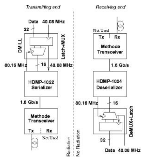
Figure 1: Single Glink Block Diagram.
