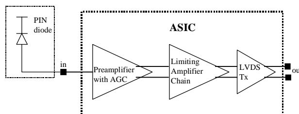
Figure 1: Schematic view of the optical receiver, which includes the PIN diode and the receiver ASIC.
