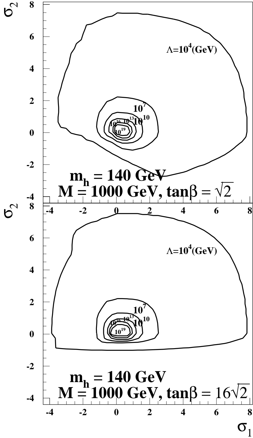
FIG. 8. The allowed range of \sigma_1 and \sigma_2 for m_h = 140 \text{ GeV} .
