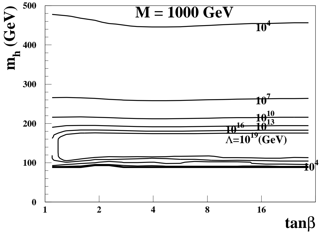
FIG. 2. The allowed mass range of the lightest CP-even Higgs boson for M = 1000 GeV. \Lambda is the cut-off scale.
