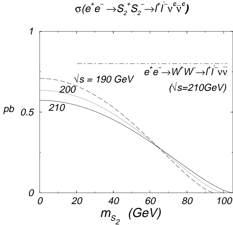
FIG. 13. The cross section of the leptonic decay process e^+e^- \rightarrow S_2^+ S_2^- \rightarrow \ell^+ \ell'^- \cancel{E}_T (where \ell and \ell' = e or \mu ) at \sqrt{s} = 190, 200, 210 GeV. The process e^+e^- \rightarrow W^+W^- \rightarrow \ell^+ \ell'^- \cancel{E}_T at \sqrt{s} = 210 GeV is shown for comparison.
