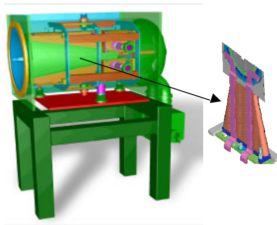
Figure 14: Vertex detector vacuum tank and detector hybrid.
