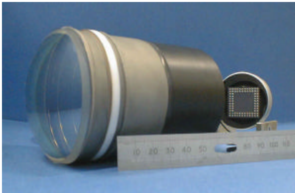
Figure 17: Pixel HPD tube
