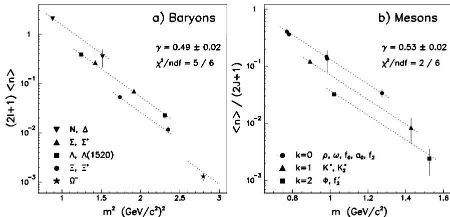
Figure 1: a) Sum of the baryon production rates of all states of an isomultiplet as a function of the squared baryon mass. b) Meson production rate per spin and isospin state as a function of the meson mass.
