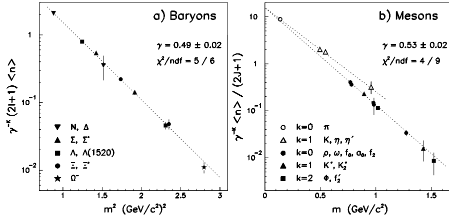
Figure 2: a) Sum of the baryon production rates of all states of an isomultiplet weighted by a factor \gamma^{-k} as a function of the squared baryon mass. b) Meson production rate per spin and isospin state weighted by a factor \gamma^{-k} as a function of the meson mass.
