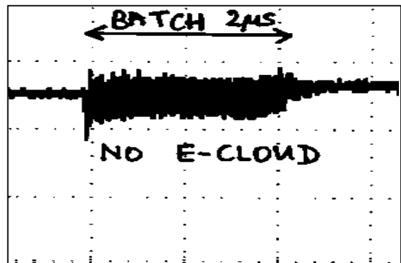
Figure 7: Vertical damper signal with a solenoid magnetic field of 100 Gauss to suppress the e'cloud ( 5.5 \times 10^{12} p/batch).
