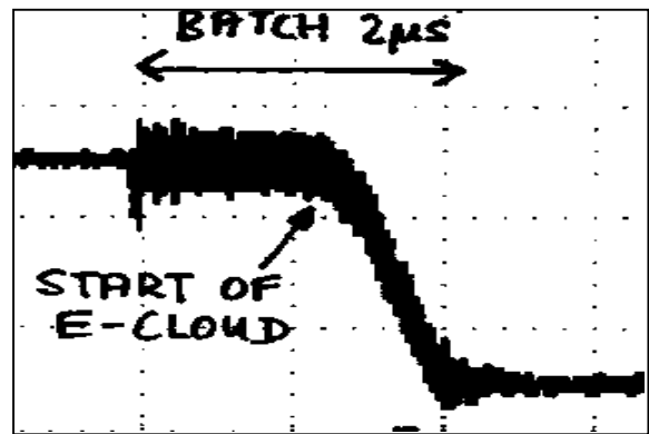
Figure 6: Vertical damper pick-up signal perturbed by the e cloud effect ( 5.5 \times 10^{12} p/batch).
