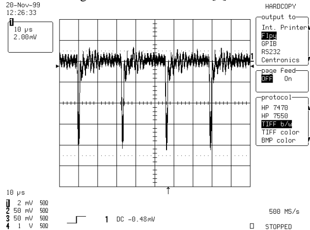
Figure 5: Structure of the current collected by the biased (+45 V) pick-up with a proton bunch density of 7.5 \times 10^{10}
