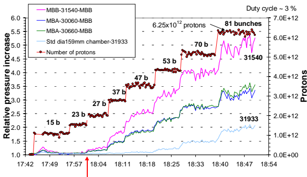
Figure 3: Relative pressure increase versus number of bunches at 7.7 \times 10^{10} p/bunch.
