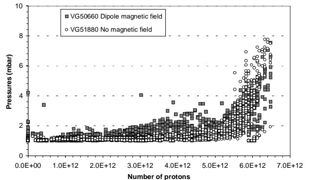
Figure 2: Pressure versus number of p/batch between two dipoles i.e. without magnetic field, duty cycle 45 %.
