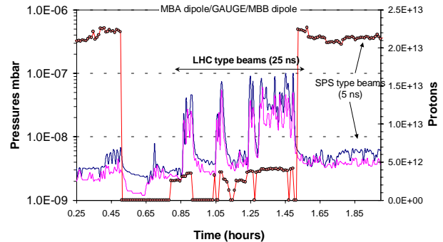
Figure 1: Pressure versus time, total number of protons= 4.5 \times 10^{12} ( 5.6 \times 10^{10} p/bunch), duty cycle 62 %.
