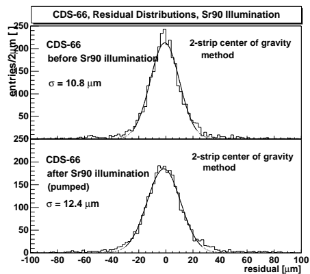
Fig. 3. Distributions of the residuals before (upper) and after (lower) electron illumination.
