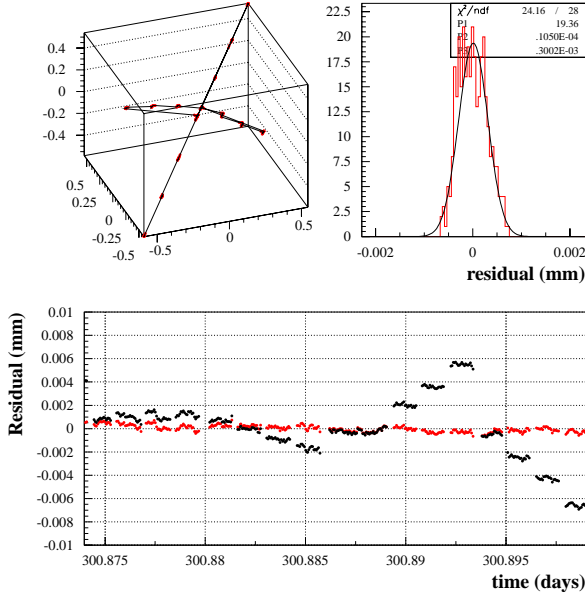
Figure 4 Results from triplet cross-calibration of BPMs.
