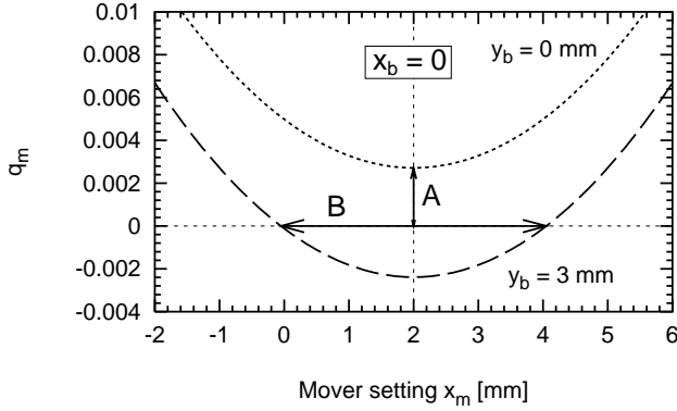
Figure 3 q_m as a function of the mover setting for example parameters. The minimum is at x_b=0 . The offset x_0 was chosen to be 2 mm in this example. The two curves correspond to different values of y_b . We use LEP parameters (BPM at QL17, 94.5 GeV, a = 4.2 cm, \sigma_x = 2.19 mm, \sigma_y = 0.06 mm).
