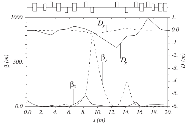
Figure 2: Optics functions of the new injection line.
