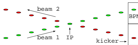
Figure 3: View of the feedback system from above. The beams collide with a fixed horizontal angle \theta_c . The BPM measures the vertical position of beam 1 and the kicker corrects beam 2 accordingly.
