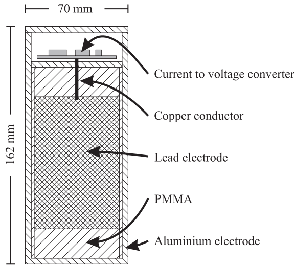
Figure 2: Layout of a Compton-diode.
