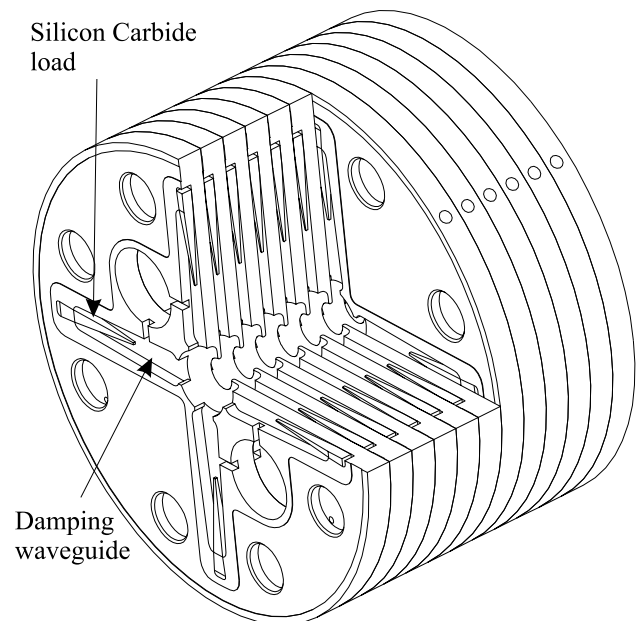
Figure 1: A cross-sectional view of the TDS cell and damping waveguide layout.
