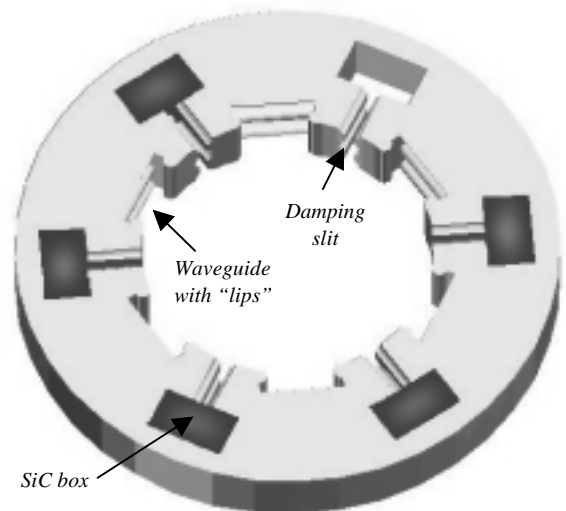
Figure 1. General layout of the PETS cross-section.
