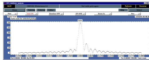
Figure 1: Tune scan.
