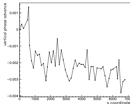
Figure 5: The effect of transverse impedance on the vertical betatron phase.
