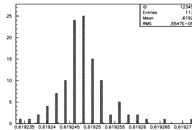
Figure 2: Tune distribution.
