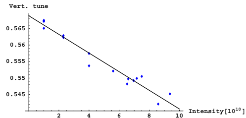
Figure 4: Vertical tune as a function of SPS beam intensity.
