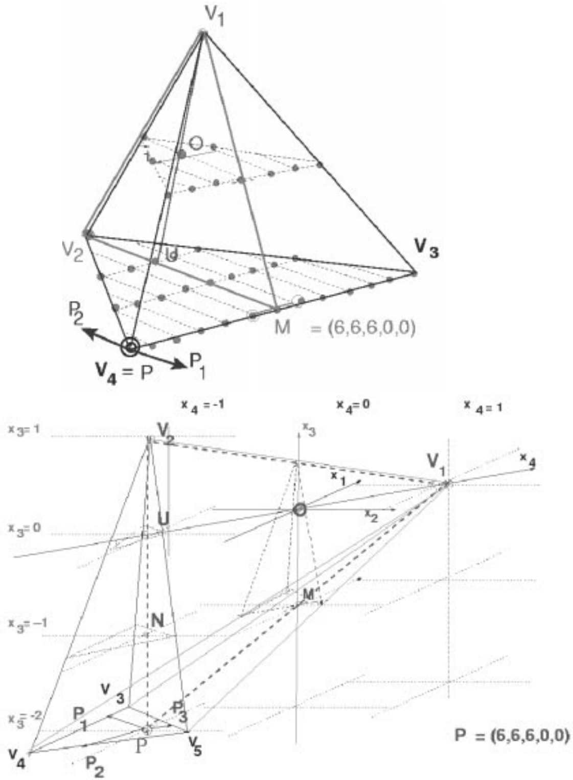
Figure 1: (a) The ‘expansion’ method for CY_3 spaces in the two-vector chain: m(1, 0, 1, 4, 6) + n(0, 1, 1, 4, 6) , which intersect in the K3 space generated by k_4 = (1, 1, 4, 6) [7], and (b) the ‘double-expansion’ method for the three-vector chain m(1, 0, 0, 2, 3) + n(0, 1, 0, 2, 3) + l(0, 0, 1, 2, 3) with an elliptic Weierstrass fibre [7], indicated by the dashed triangle. The double-expansion point for this chain is P = (6, 6, 6, 0, 0) .
