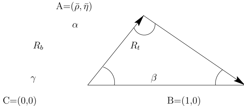
Figure 1: Unitarity Triangle.
