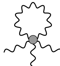
Figure 1: Feynman diagram involving the vertex V_M^{(5)} (shaded circle) that derives from the measure term. The diagram appears at two-loop order, while all other diagrams with such vertices and less than four external lines are of higher order.
