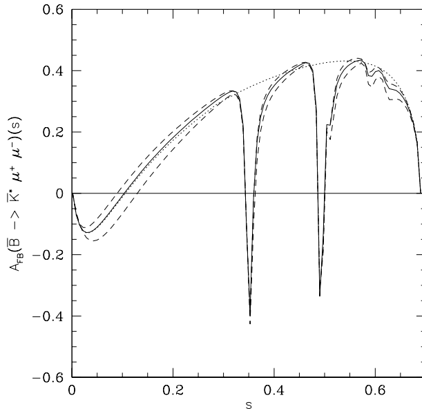
Figure 4: Forward-backward asymmetry for \bar{B} \rightarrow \bar{K}^* \mu^+ \mu^- , defined as in (59). The solid (dotted) curves have been obtained employing the Krüger-Sehgal approach (using C_9^{\text{eff}}(s) \equiv C_9^{\text{EP}}(s) ). The dashed lines show the effect of varying the renormalization scale of the Wilson Coefficients between m_b/2 and 2m_b , within the Krüger-Sehgal approach.
