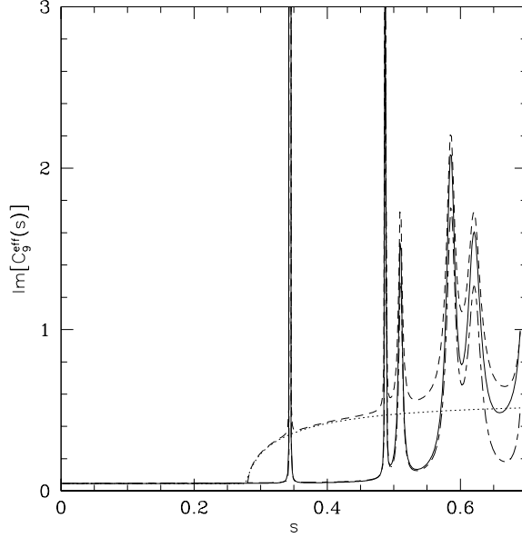
Figure 3: The imaginary part of C_9^{\text{eff}} as a function of s : \text{Im}C_9^{\text{eff}}(s) = \text{Im}C_9^{\text{EP}}(s) as in (44) (dotted); KS prescription [43] (solid); Ref. [45] (dot-dashed). For comparison we have also included the approach of Ref. [44] (dashed), where Breit-Wigner resonances are naively added to the partonic calculation. (This procedure is disfavoured since it has a manifest problem of double-counting.)
