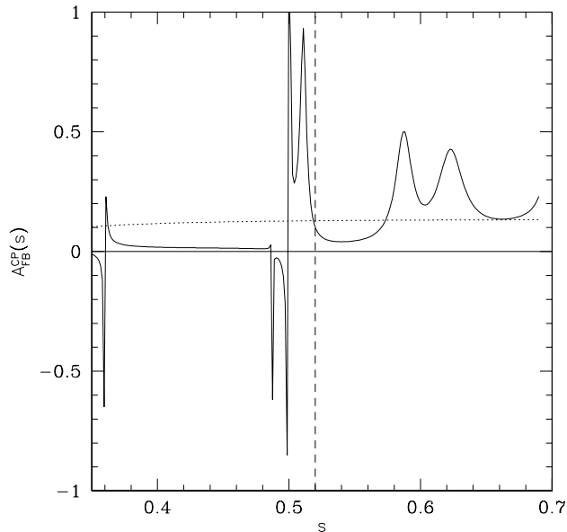
Figure 5: The forward-backward CP asymmetry defined in (63), in units of \text{Im}C_{10}/\text{Re}C_{10} , as a function of s . Solid and dotted lines correspond to the Krüger-Sehgal approach and to the choice C_9^{\text{eff}}(s) \equiv C_9^{\text{EP}}(s) , respectively. The vertical dashed line denotes the lower limit of the integration range in (66).
