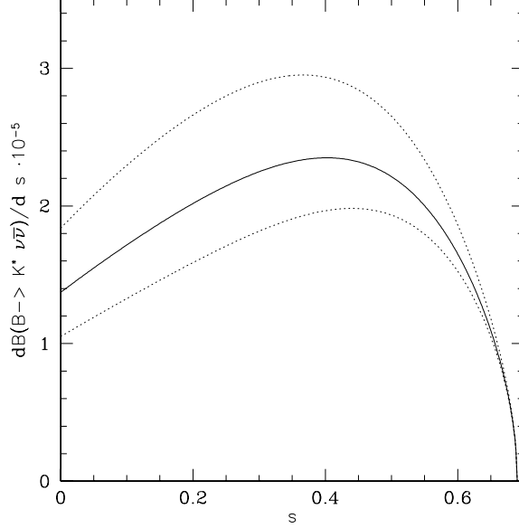
Figure 2: Dilepton invariant mass distribution for \mathcal{B}(B \rightarrow K^* \nu \bar{\nu}) within the SM. The three lines correspond to the central, minimal and maximal values, as obtained by varying the form factors within the ranges quoted in [19].
