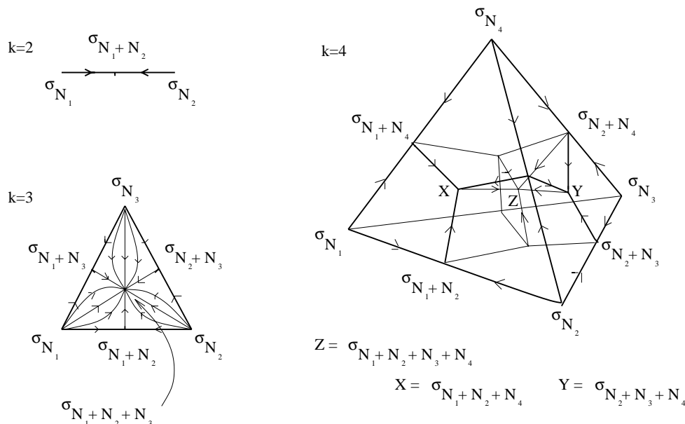
Figure 3: Polyhedral RG patterns interpolating between pairs of \sigma_N models.
