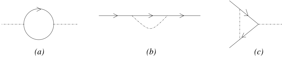
Figure 1: Leading diagram and first subleading corrections.
