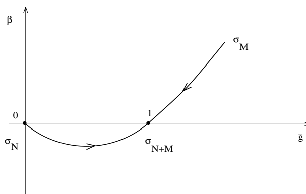
Figure 2: Beta function of dual RG flows.
