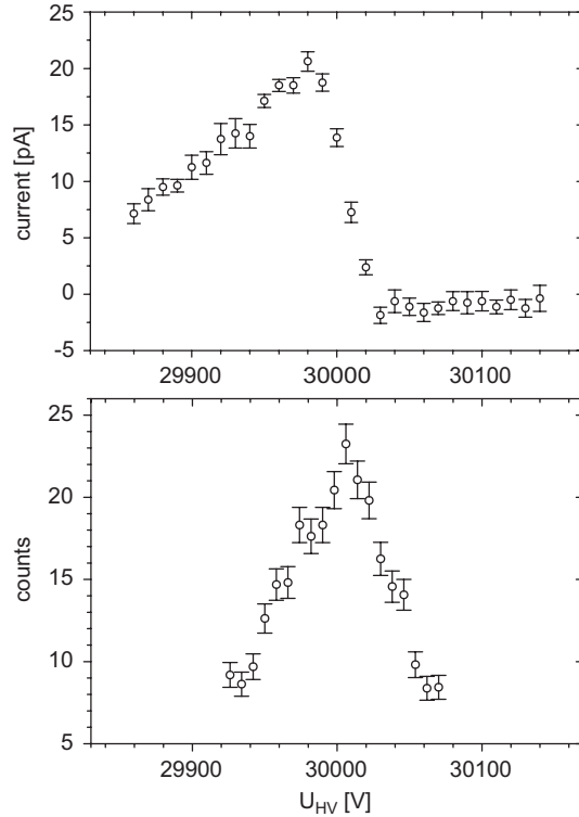
Fig. 18. Current of ^{132}\text{Xe}^+ ions guided through the RFQ (top) and number of accumulated and ejected ions in bunching mode (bottom) as a function of the voltage U_{HV} of the HV platform.
