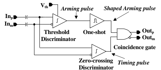
Fig. 7: Discriminator block diagram
