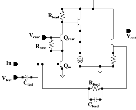
Fig. 2: Current Preamplifier
