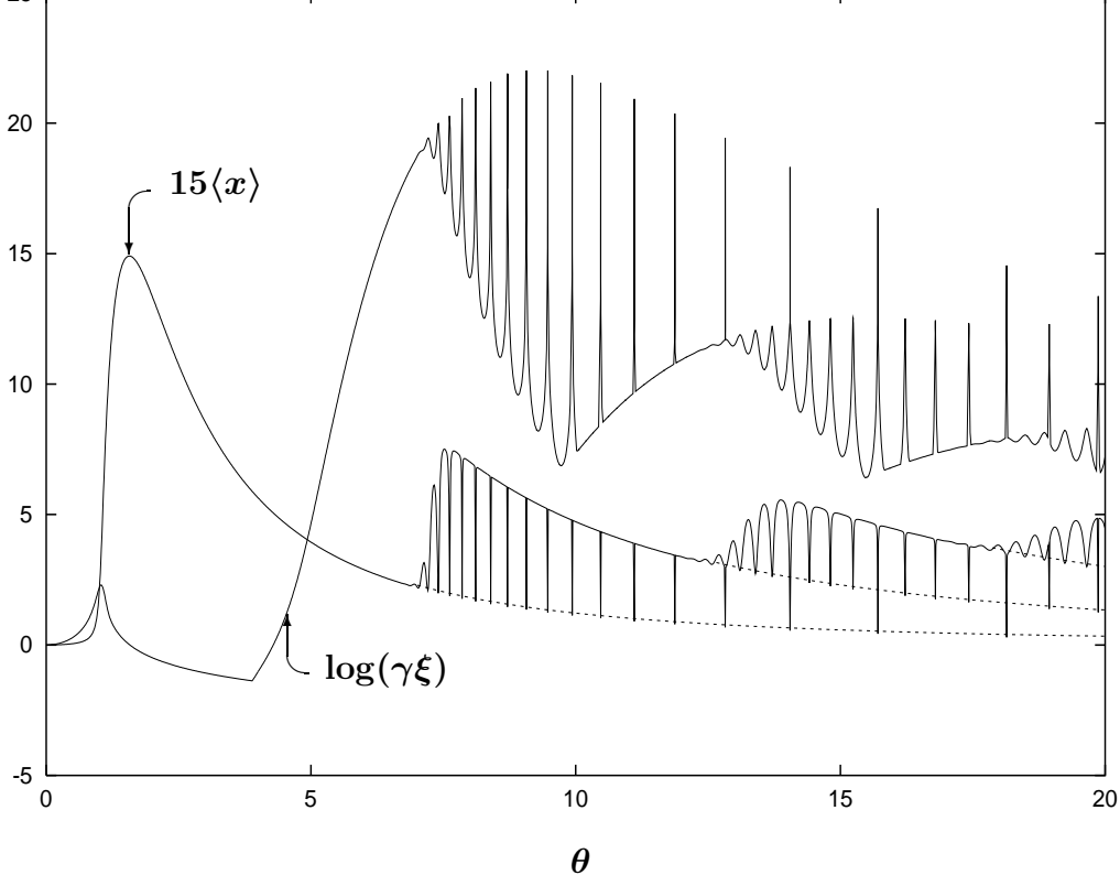
Figure 15: The logarithm of \gamma\xi and 15\langle x \rangle as a function of \theta when the parameters are as in Fig. 13. There is no visible difference between the \theta -positions of the correlation trapping-peaks and the \theta -positions of the order parameter trapping-dips. The dotted lines are the mean field solution Eq. (26) and Eq. (27) for branch k = 0 , k = 1 and k = 2 for some limited interval of \phi .
