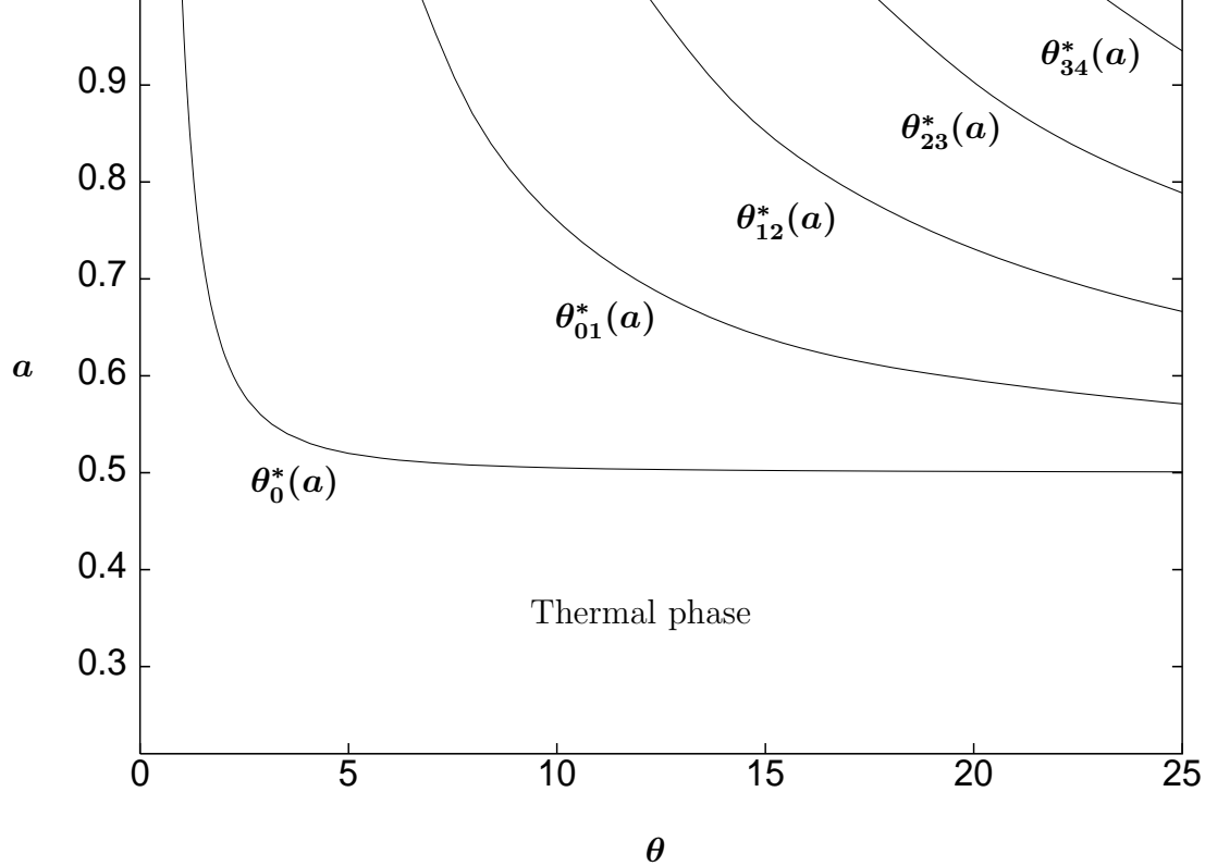
Figure 3: The phase diagram for the micromaser system when n_b = 0.15 and \Delta = 0 . All the critical lines converge to 1/2 in the large \theta limit. The thermal-to-maser critical line \theta_0^*(a) is determined analytically by Eq. (43). The other critical lines \theta_{kk+1}^*(a) , which are maser-to-maser transitions, are determined by Eq. (52).
