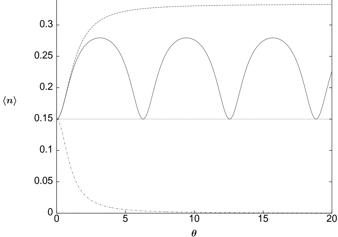
Figure 5: This figure shows the different behaviours of Eq. (65). n_b = 0.15 for all curves. The straight line corresponds to a = n_b/(1 + 2n_b) = 3/26 , i.e. thermal equilibrium. The solid curve corresponds to a = 0.2 and |\Delta| = 0.5 . The fat dotted curve corresponds to a = 0.2 and \Delta = 0 . The dashed-dotted curve corresponds to a = 0 and \Delta = 0 .
