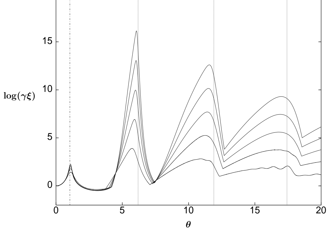
Figure 8: The logarithm of the correlation length \gamma\xi as a function of \theta for various values of N = 25, 50, \dots, 125 when n_b = 0.15 , |\Delta| = 0.5 and a = 1 . The numerical values of the vertical lines are as in Fig. 2.
