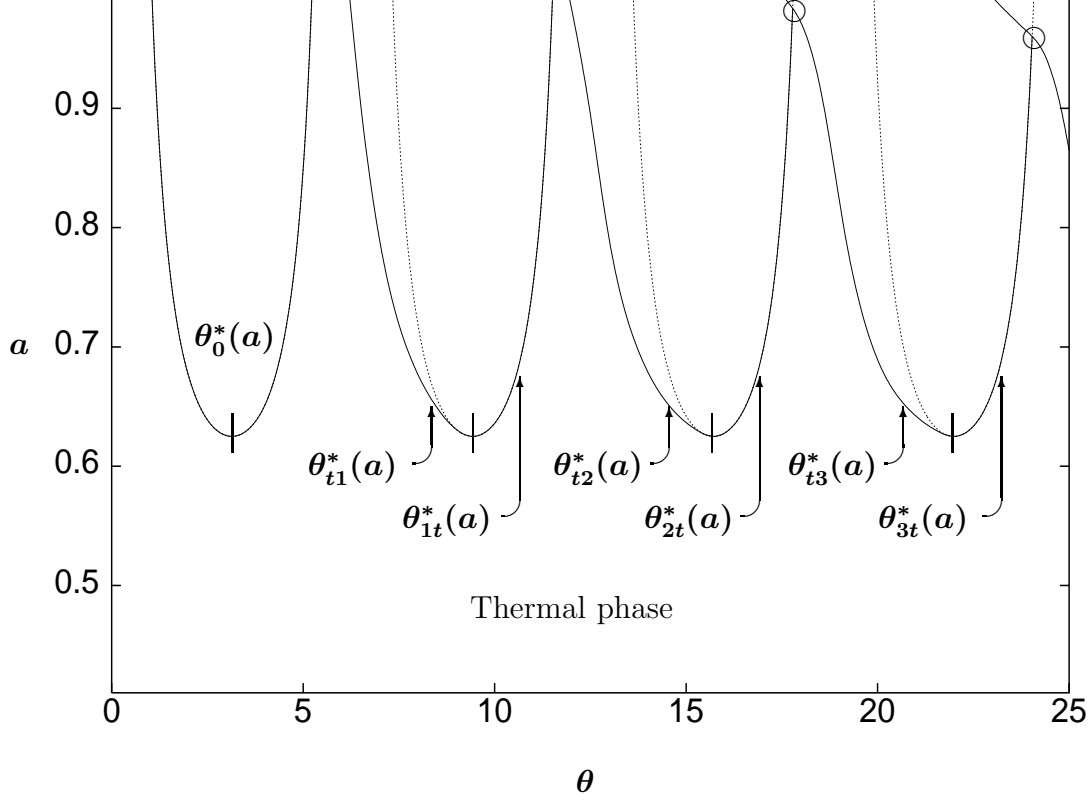
Figure 4: The phase diagram for the micromaser system when n_b = 0.15 and |\Delta| = 0.5 . In this diagram we have plotted the range of validity of the thermal distribution (dotted lines). When not visible these dotted lines overlap with the solid critical lines. The minima of the critical lines are determined by the condition \sin^2(\Delta\theta) = 1 and are marked by a short vertical lines. The first critical line \theta_0^*(a) in this phase diagram is determined analytically by Eq. (41). The critical lines \theta_{tk}^*(a) are given by Eq. (55) and \theta_{kt}^*(a) are given by Eq. (59). Triple points are indicated by circles. The numerical values of these triple points are (a_{23}, \theta_{23})^{triple} = (0.98, 17.78) and (a_{34}, \theta_{34})^{triple} = (0.96, 24.04) .
