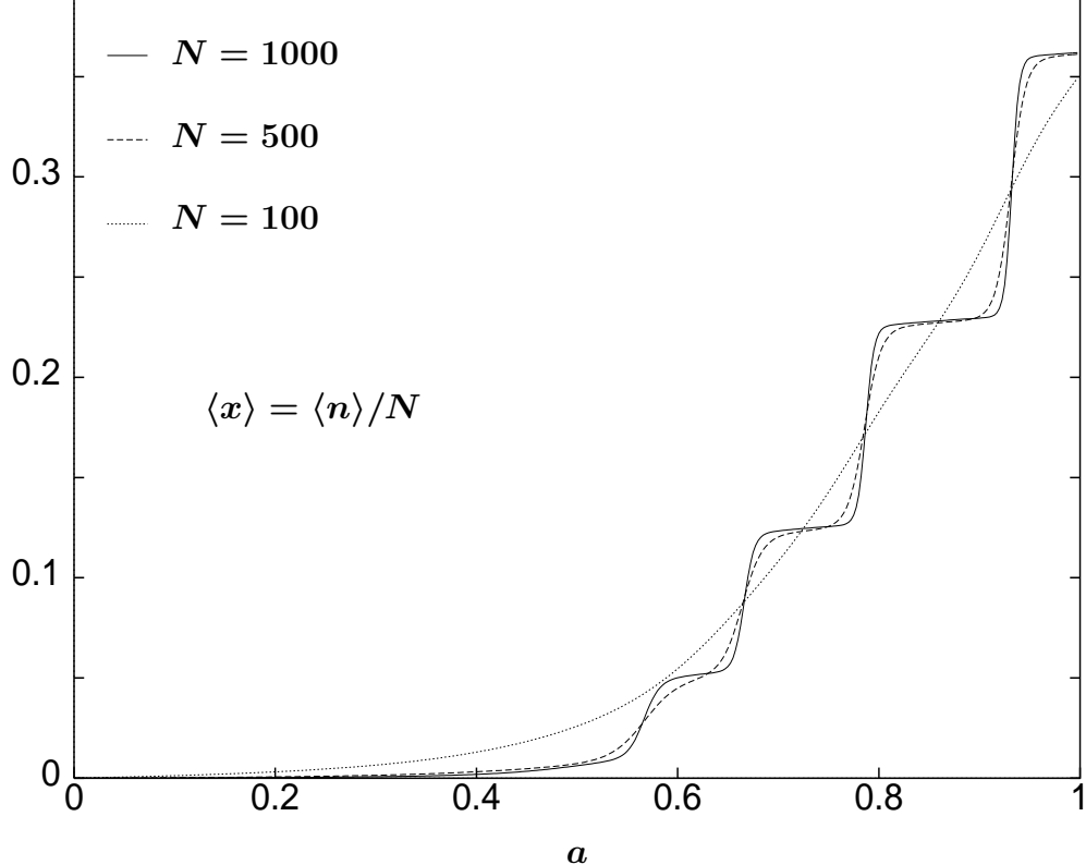
Figure 6: The order parameter \langle x \rangle = \langle n \rangle / N as a function of a when n_b = 0.15 , \Delta = 0 , \theta = 25 and N = 100, 500, 1000 . Each step in \langle x \rangle corresponds to a point on one of the transition curves in Fig. 3.
