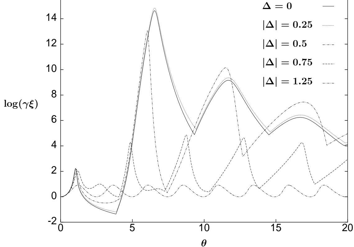
Figure 9: The logarithm of the correlation length \gamma\xi as a function of \theta for various values of |\Delta| = 0, 0.25, 0.50, 0.75 and 1.25 when n_b = 0.15 , a = 1 and N = 100 .
