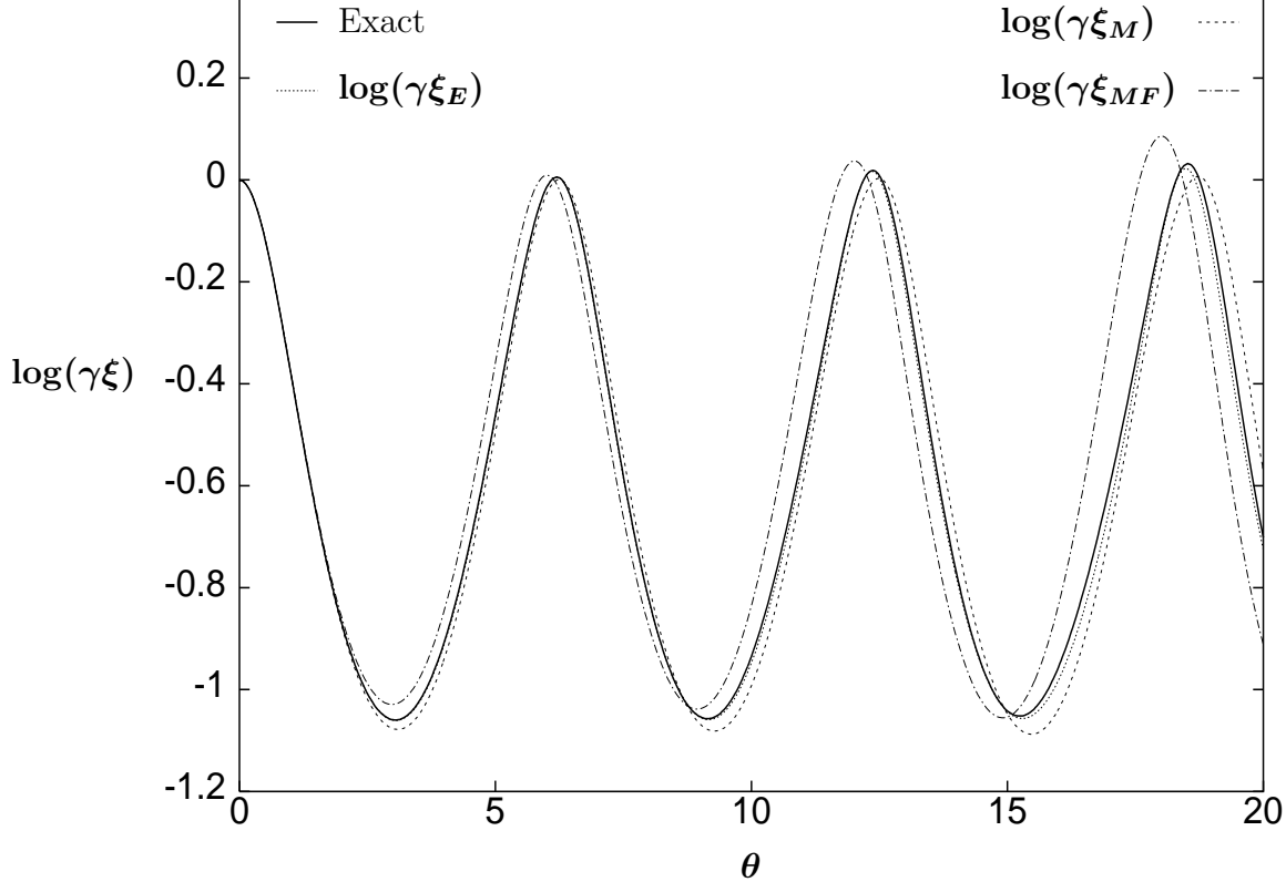
Figure 12: Comparison of \log(\gamma\xi) as a function of \theta for various analytical expressions of the correlation as derived in the text. The parameters for all curves are a = 0.25 , |\Delta| = 0.5 , n_b = 0.15 and N = 100 . The solid curve is the exact correlation length. In the large N limit all curves overlap completely.
