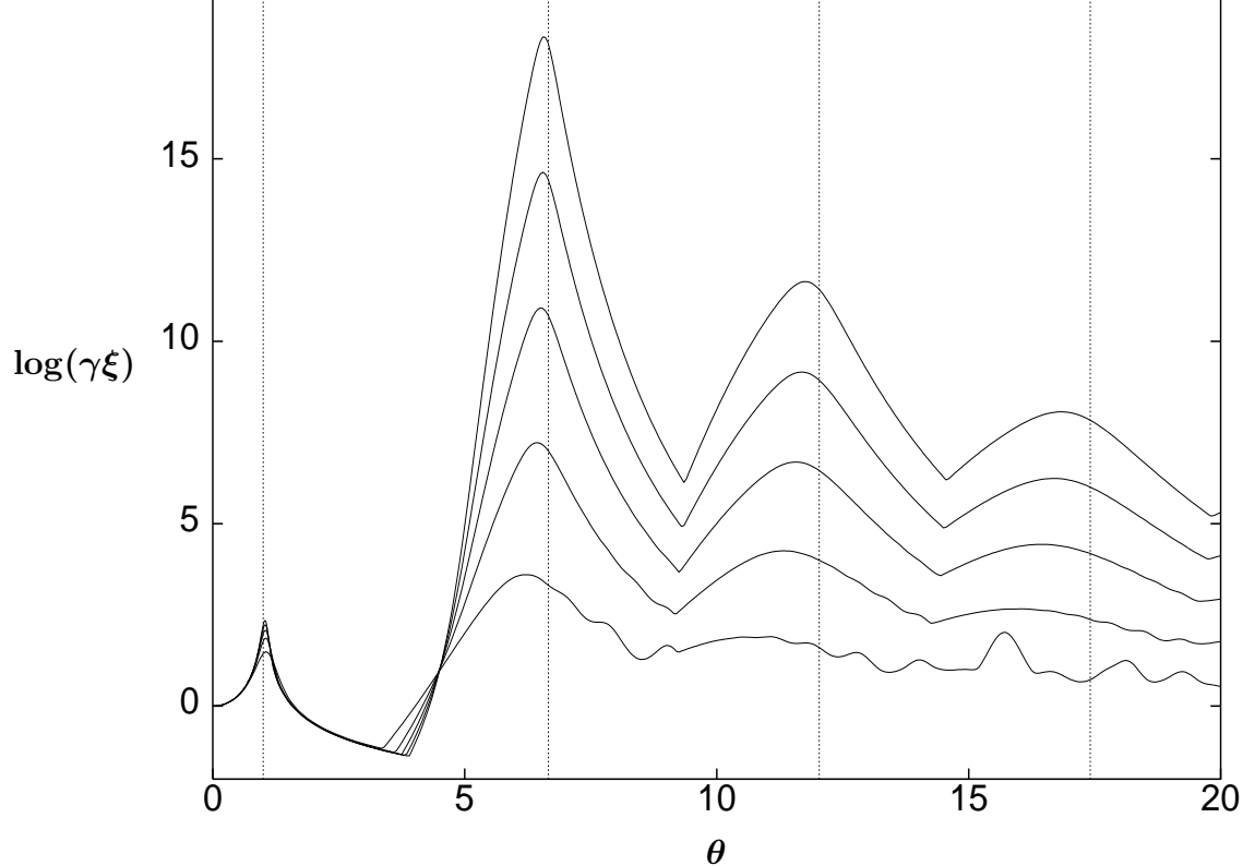
Figure 7: The logarithm of the correlation length \gamma\xi as a function of \theta for various values of N = 25, 50, \dots, 125 when n_b = 0.15 , \Delta = 0 and a = 1 . The numerical values of the vertical lines are as in Fig. 1.
