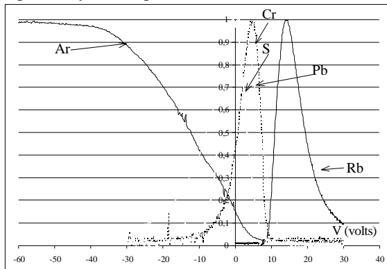
Fig. 2 : Relative 1+ \rightarrow n+ efficiency versus V .
