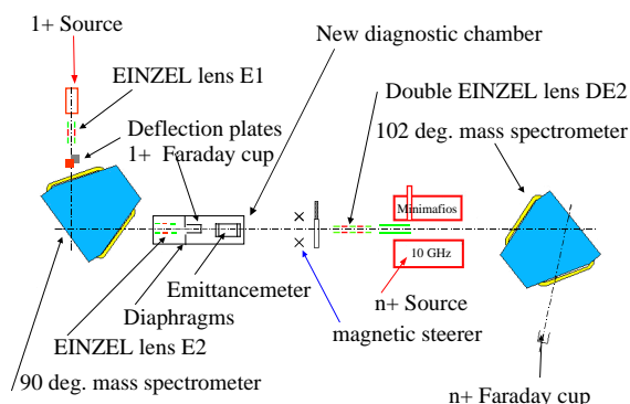
Fig. 1: 1+ \quad n+ experimental setup.
