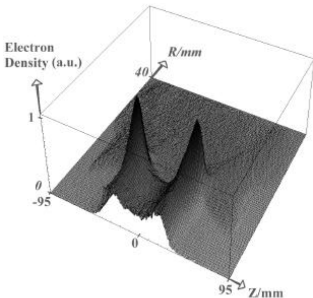
Fig. 15b. The azimuthally averaged electron density in ECRIS III (14 GHz)
