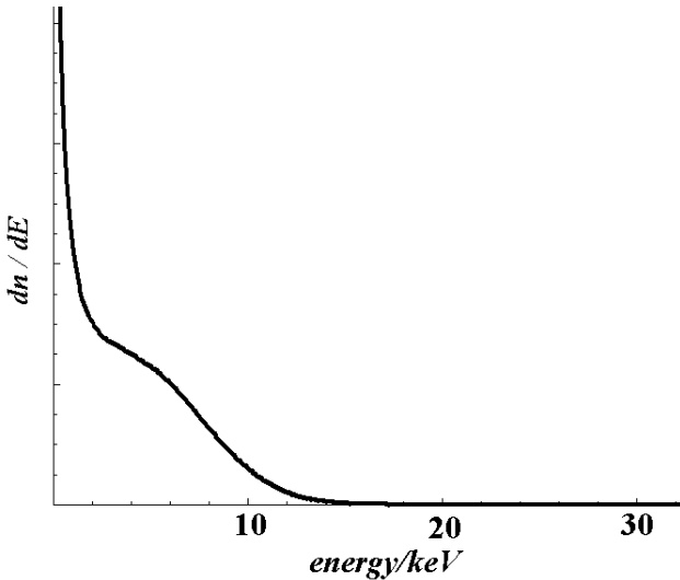
Fig. 10. Electron energy spectrum in the regions of high energy density in ECRIS III - H_{113} at 100 V/cm
