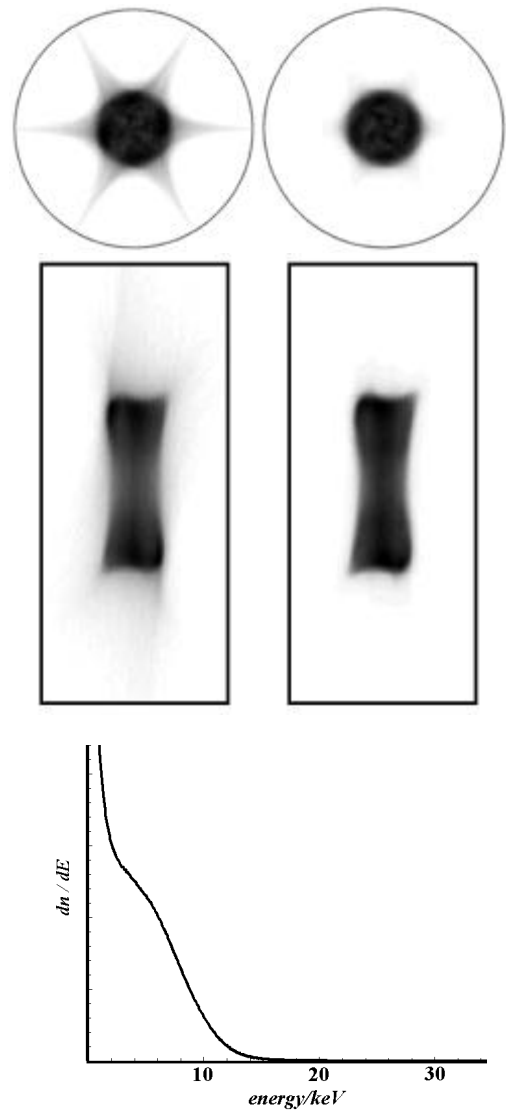
Fig. 16. Same as Fig.15 but run with a single frequency in resonance at the center of the resonance volume.
