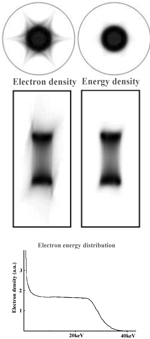
Fig. 15. Projections of the electron distributions of ECRIS III (14 GHz) along the symmetry z -axis (top) and along the y -axis (bottom). Left: Density. Right: Energy density. The source is run with 23 frequencies as indicated in Fig.14 with a field of 100 V/cm each. Simulation time: 1 \mu s
