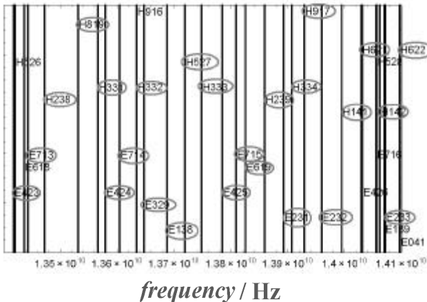
Fig. 14. Spectrum of resonance frequencies of a cavity 80 mm diameter x 190 mm length near 14 GHz
