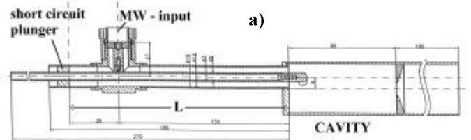
Fig. 3a. 6.7 GHz MW coupling into the plasma cavity.
