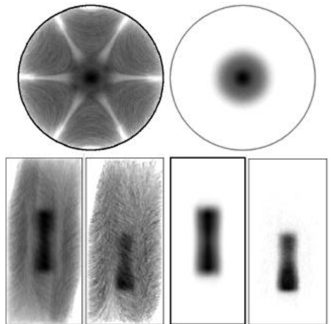
Fig. 8. Projections of the electron distributions of ECRIS III - H_{113} along the symmetry z -axis (top) and along the y -axis (bottom). Left: Density. Right: Energy density. Every second subfigure at the bottom represents the results of ECRIS IIIS.
