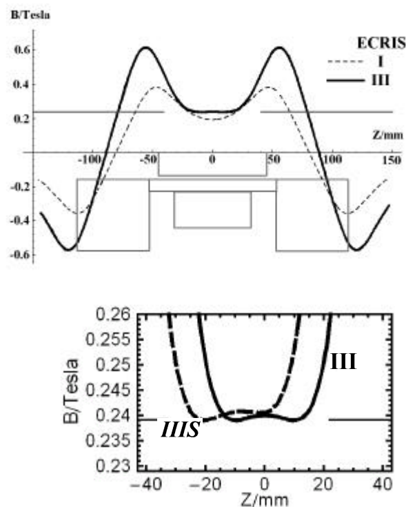
Fig. 1. Magnetic field components B_z on the axis of symmetry of ECRIS I and III with the positions of the radially magnetized rings, the hexapole and the plasma chamber.
