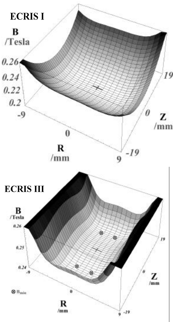
Fig. 2. Magnetic confinement and resonance volume of ECRIS I and ECRIS III.
