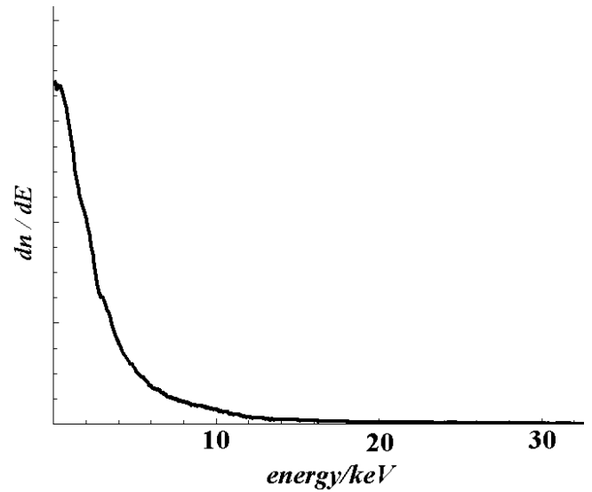
Fig. 7. Electron energy spectrum in the regions of high energy density in ECRIS I - H_{113}
