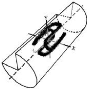
Fig. 6. Typical trajectory wound in loops forming the densities in Fig.5
