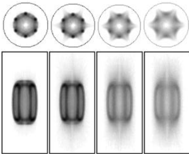
Fig. 17. The afterglow: Projections of the electron density distributions of ECRIS I along the symmetry z -axis (top) and along the y -axis (bottom). From left to right: Before switch off, 0.25 ms, 2 ms, and 4 ms after switch off of the MW
