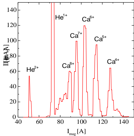
Fig.4. ^{48}\text{Ca} ion spectrum produced from the metallic calcium. He is used as a support gas.
