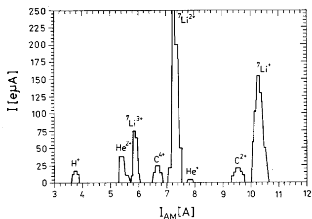
Fig.1 Li ion spectrum optimized for \text{Li}^{2+} production. He is used as a support gas.
