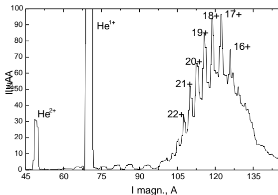
Fig.5. Bi ion spectrum. He is used as a support gas.
