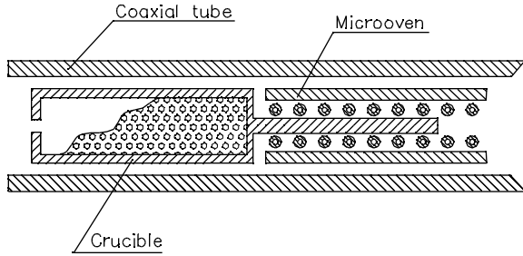
Fig.2 Schematic view of the large volume crucible for Mg ion production.
