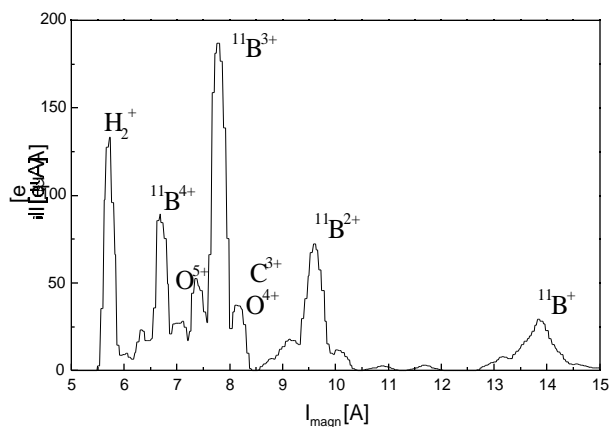
Fig.5 The spectrum of boron ions produced from \text{C}_2\text{B}_{10}\text{H}_{12} compound.
