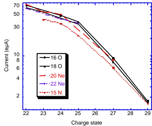
Fig. 4 – Krypton current with different oxygen isotope.
