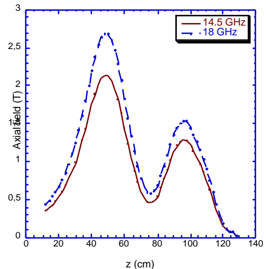
Fig. 2 – Axial magnetic field of SERSE.
