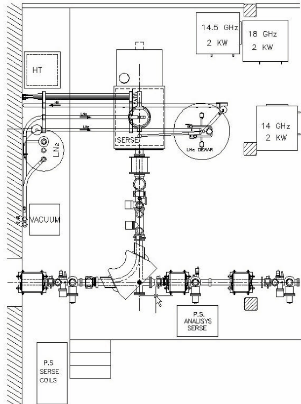
Fig. 5 - SERSE with the analysis section of the beamline.
