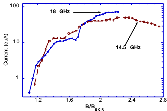
Fig. 6 – \text{Xe}^{27+} currents vs. B_{\text{radial}}/B_{\text{ECR}} .
