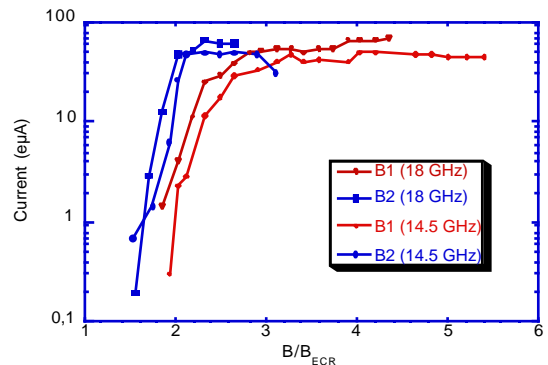
Fig. 7 – \text{Xe}^{27+} currents vs. B_{\text{axial}}/B_{\text{ECR}} on injection (1) and extraction side (2).
