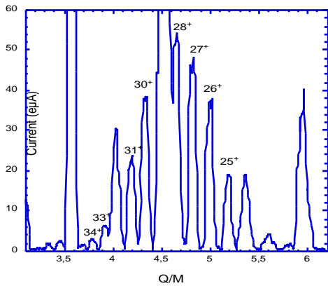
Fig. 3 – Charge state distribution for Xe, optimized for 30 + .
