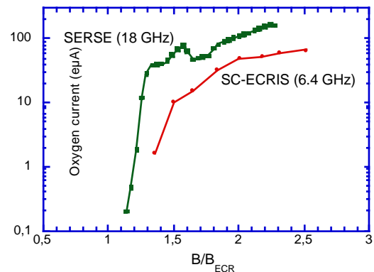
Fig. 8 – \text{O}^{7+} current vs. B_{\text{radial}}/B_{\text{ECR}} .
