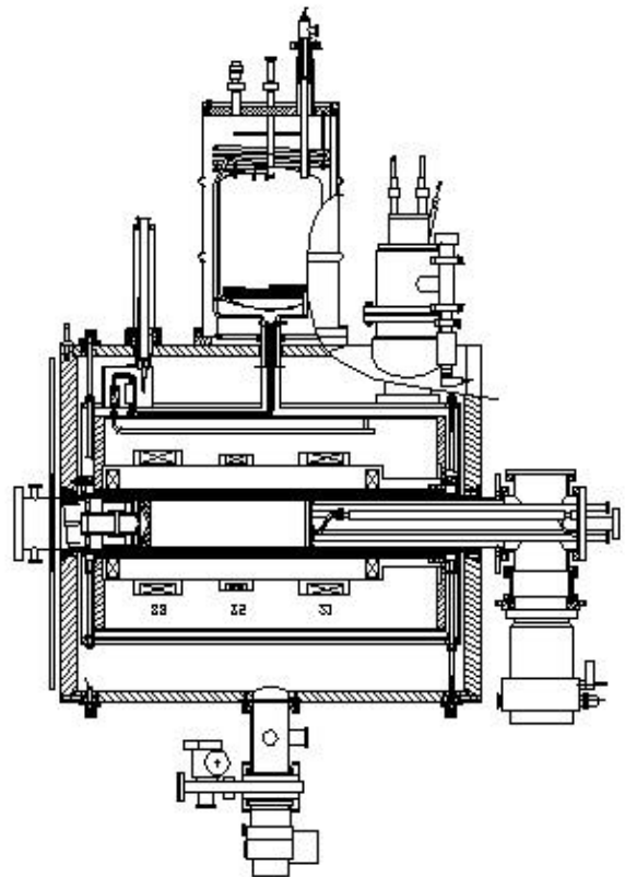
Fig. 1 - The SERSE source.
