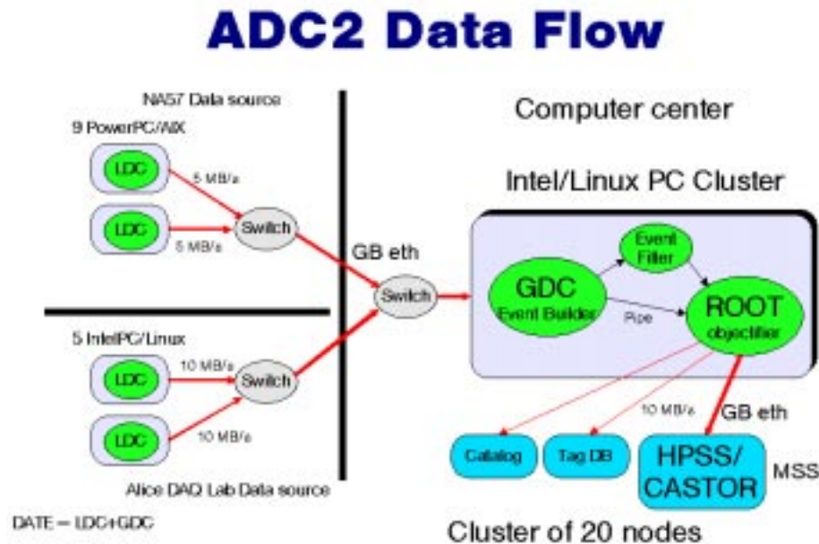
Figure 2: The planned ADC2 setup
