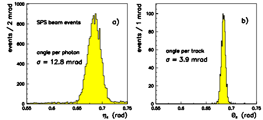
Figure 8. Photon angle (a) and track Cherenkov angle (b) distributions for beam events at the SPS. The distribution (b) has been obtained considering only photons with 0.55 < \eta_c < 0.75 rad to shorten the computing time.
