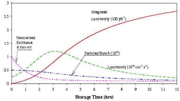
Figure 2. Beam parameters during a store for high-field VLHC.
