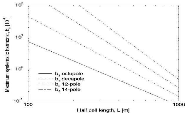
Figure 1. Maximum allowable systematic harmonics vs. half cell length, when \Delta Q_x = 0.1 , \phi_c = 90 degrees, \epsilon_x = 1 \mu\text{m} , at an energy of 1 TeV, with a reference radius of 16 mm
