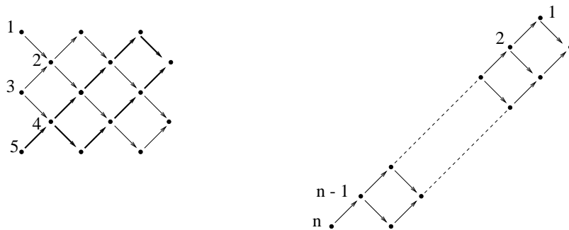
Figure 1: Paths in \mathbb{A}_5 and \mathbb{A}_n
