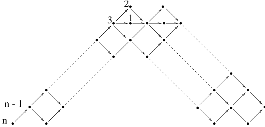
Figure 2: Paths in \mathbb{D}_n
