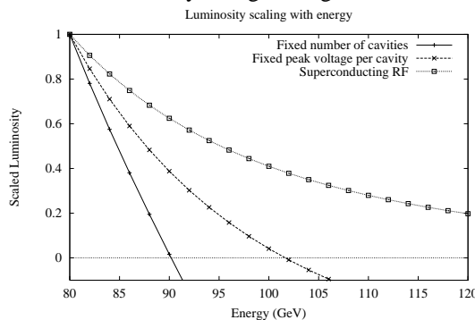
Figure 3, Luminosity for different rf options.
