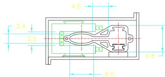
Figure 2. The magnet, vacuum chamber and support.
