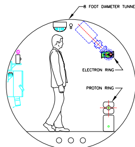
Figure 1, The collider rings in the tunnel.
