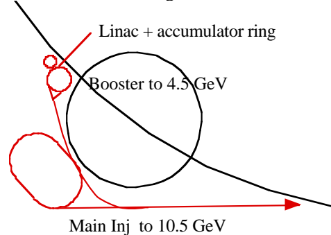
Figure 4. An electron injector chain.
