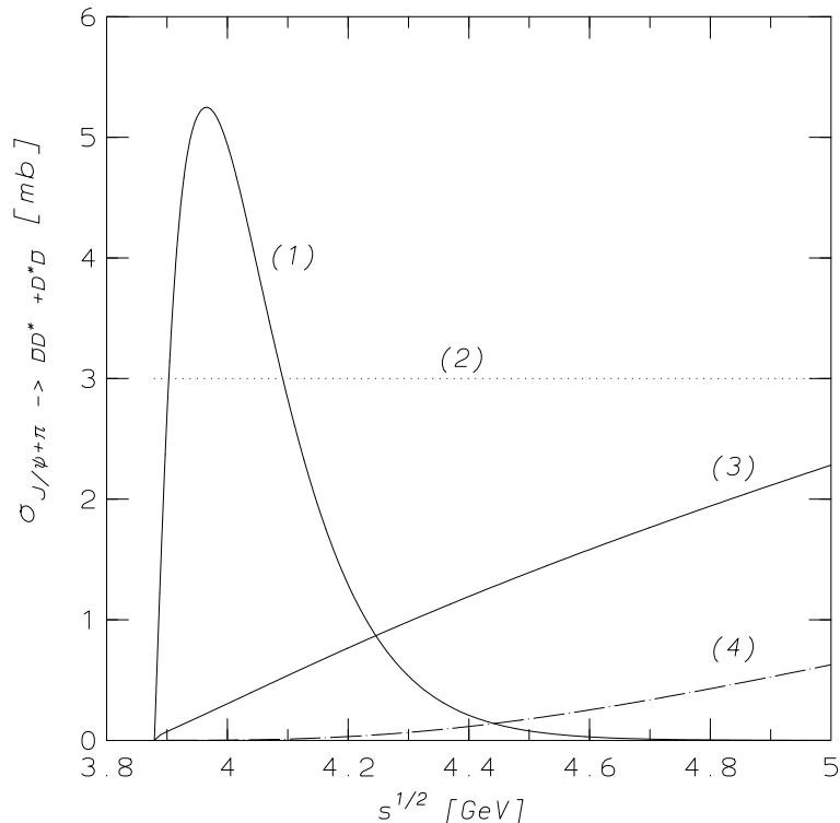
Figure 1: The cross section for J/\psi + \pi \rightarrow \bar{D}D^* + \bar{D}^*D absorption as a function of energy: curve (1) is calculated within a non-perturbative quark exchange model [4]; curve (2) corresponds to the constant cross section of 3 mb [5,6]; curve (3) was obtained within the framework of a meson exchange model [7]; curve (4) is derived in the context of perturbative QCD [8].
