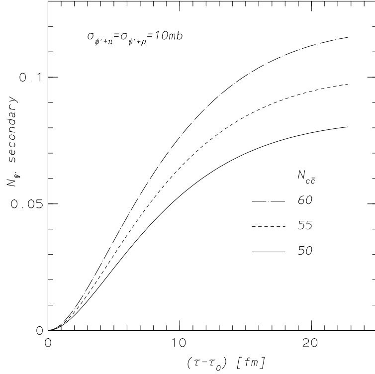
Figure 9: As in fig. 8 but for different values of the number of D\bar{D} mesons.
