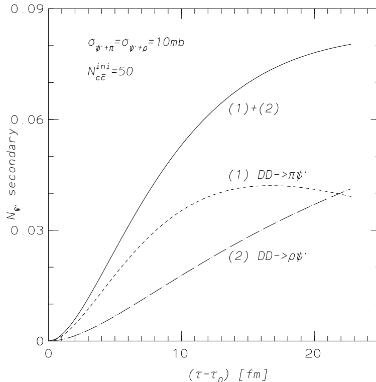
Figure 8: Time evolution of the abundance of \psi' from Pb-Pb collisions at LHC using constant absorption cross sections for \psi' - \pi and \psi' - \rho of 10 mb.
