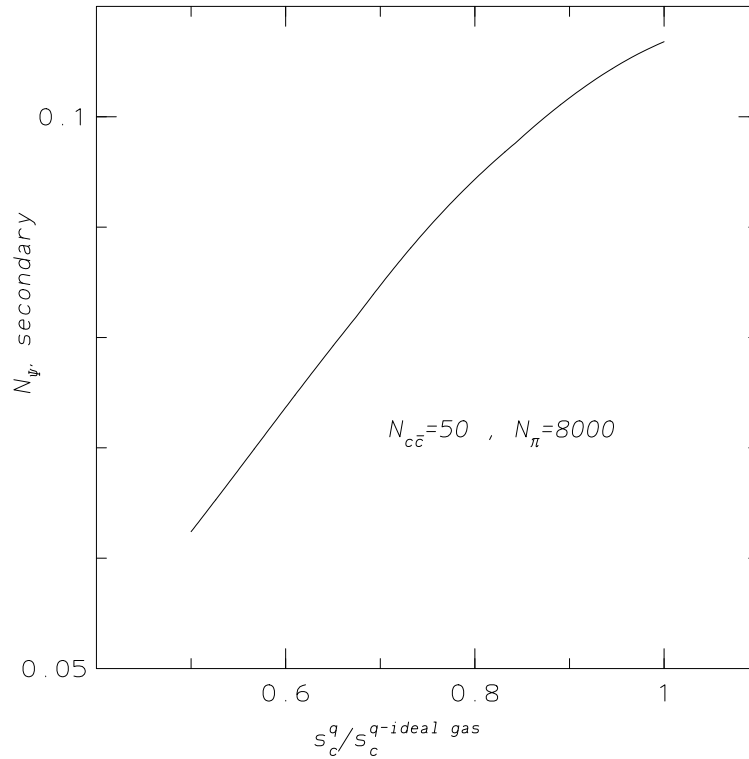
Figure 11: Total \psi' yield produced during the mixed phase as a function of the fractions of the critical entropy density of the non-interacting quark-gluon plasma.
