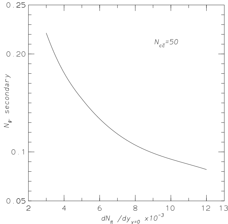
Figure 10: Total \psi' yield produced during the mixed phase as a function of pion multiplicity.
