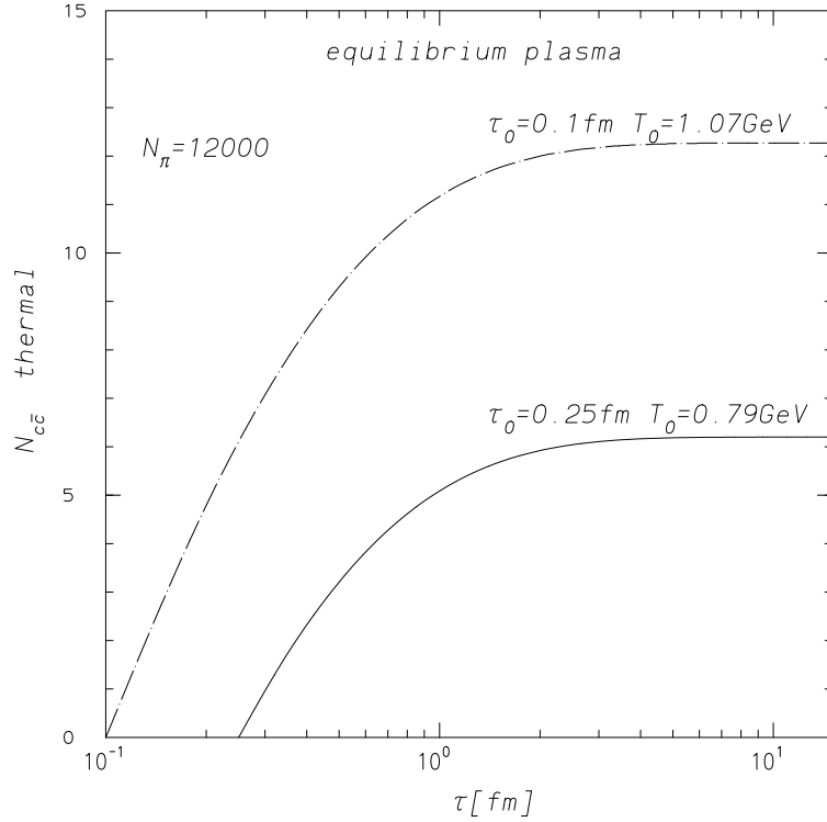
Figure 4: Time evolution of the number of c\bar{c} produced in an equilibrium QGP for two different values of the initial thermalization time and the initial temperature calculated with 12000 pions in the final state.
