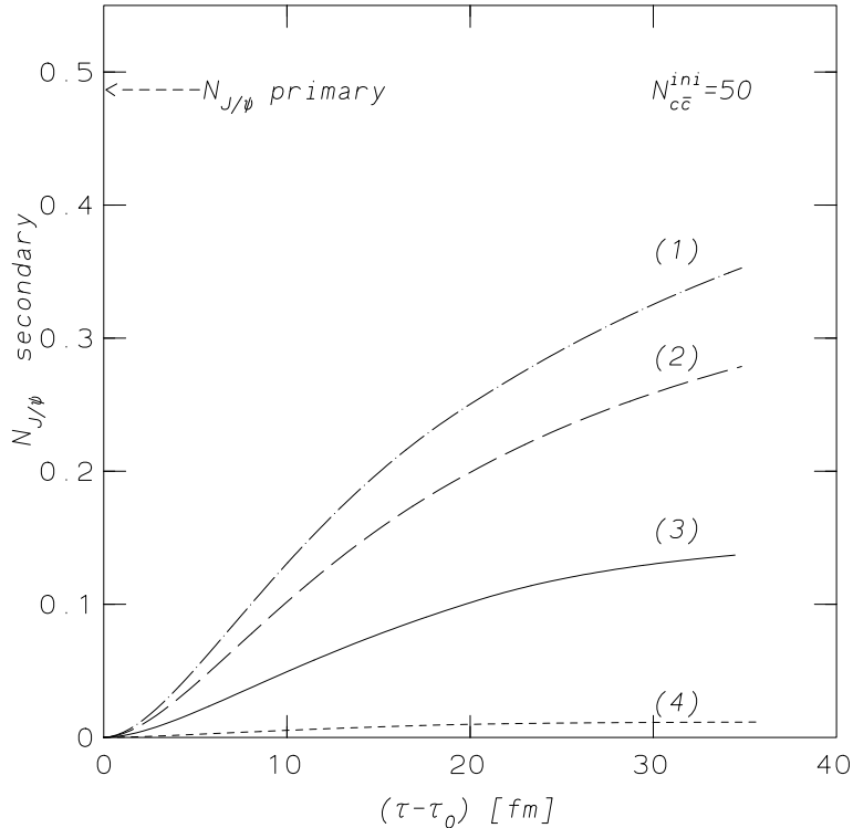
Figure 7: Time evolution of J/\psi production from hadron gas due to \bar{D}D^* + D\bar{D}^* \rightarrow J/\psi\pi process calculated for Pb-Pb collisions at LHC energy for four different parameterizations of the J/\psi - \pi absorption cross sections as described in fig. 1.
