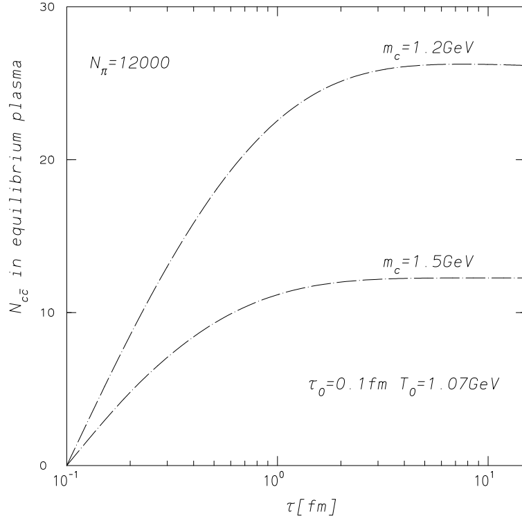
Figure 5: Time evolution of the number of c\bar{c} produced in an equilibrium QGP for two different values of the charm quark mass.
