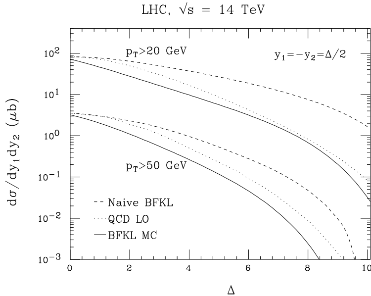
Figure 1. BFKL and asymptotic QCD leading-order dijet production cross sections at the LHC ( \sqrt{s} = 14 TeV) as a function of the dijet rapidity separation \Delta \equiv \Delta y . The three curves at each transverse momentum threshold use: (i) improved BFKL MC with running \alpha_s (solid lines), (ii) leading-order BFKL (dashed lines), and (iii) the asymptotic ( \Delta y \gg 1 ) form of QCD leading order (dotted lines).
