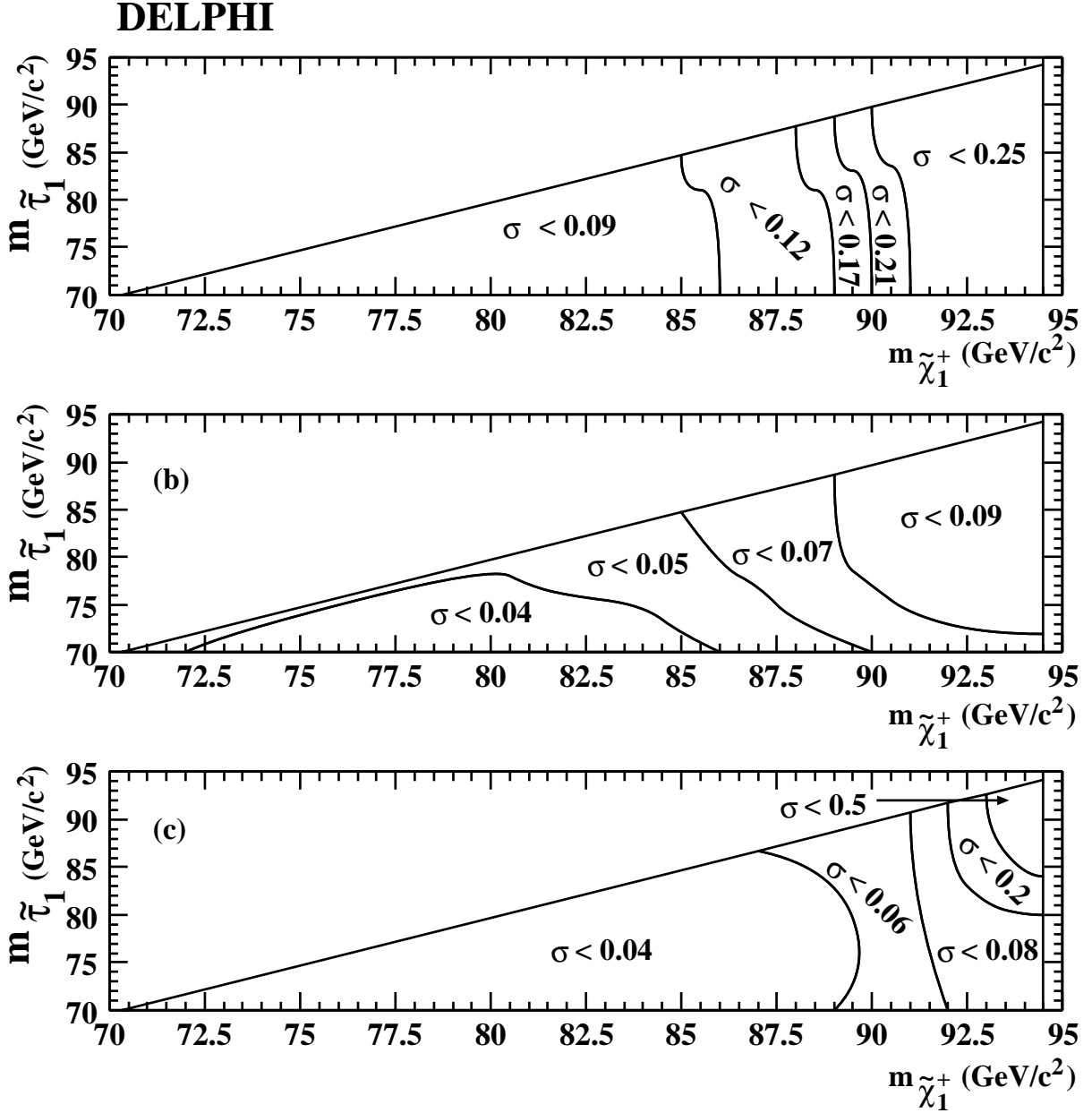
Figure 2: Limits in picobarn on the lightest chargino pair production cross-section at 95% CL. Limits are shown as functions of m_{\tilde{\chi}_1^+} and m_{\tilde{\tau}_1} for (a) m_{\tilde{G}} = 1 \text{ eV}/c^2 , (b) m_{\tilde{G}} = 100 \text{ eV}/c^2 and (c) m_{\tilde{G}} = 1000 \text{ eV}/c^2 .
